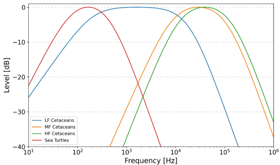
Figure A-3. Auditory weighting functions for functional marine mammal hearing groups as recommended by NMFS (2018) and Finneran et al. (2017)
