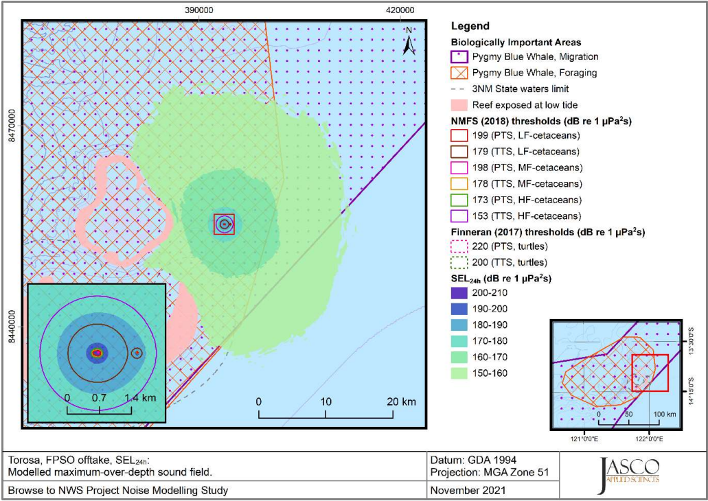
Figure 34. Torosa location, FPSO Offtake , SEL 24h : Sound level contour map showing unweighted maximum-over-depth SEL 24h results, along with isopleths for PTS and TTS thresholds in low, mid, and high-frequency cetaceans and sea turtles.
