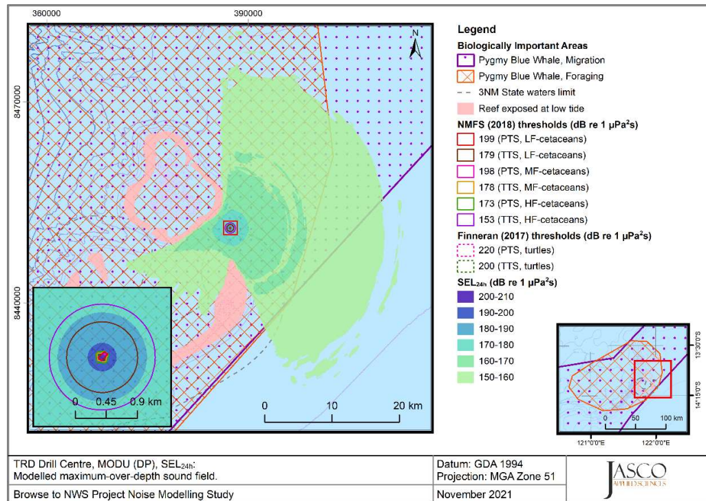
Figure 26. TRD Drill centre, MODU (DP), SEL 24h : Sound level contour map showing unweighted maximum-over-depth SEL 24h results, along with isopleths for PTS and TTS thresholds in low, mid, and high-frequency cetaceans and sea turtles.
