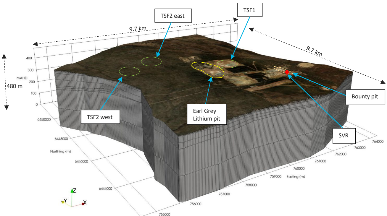
Figure 3.1 Model domain (vertical exaggeration x 5)
