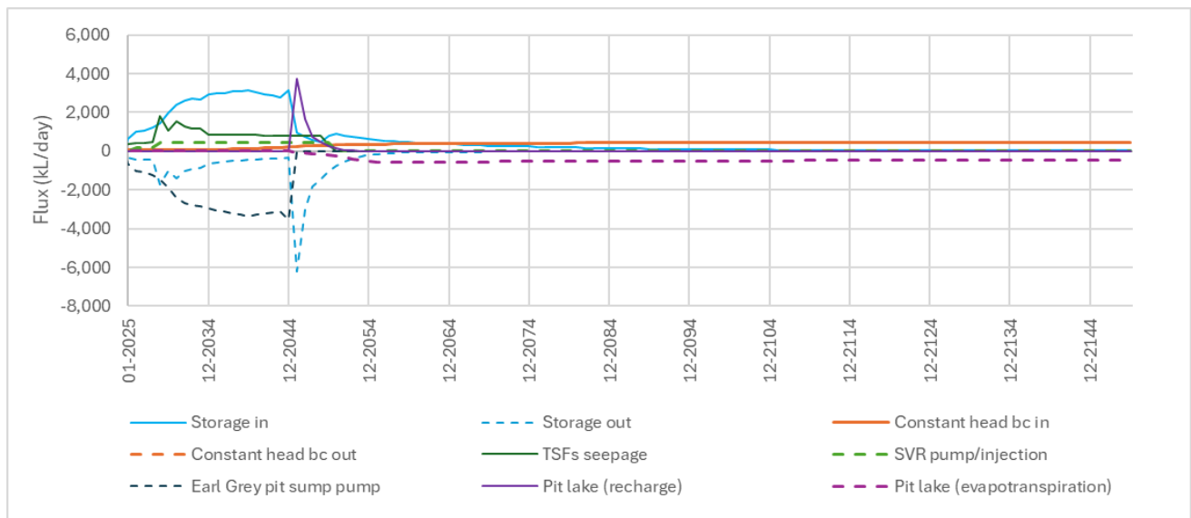
Figure 5.2 Water balance during predictive period
