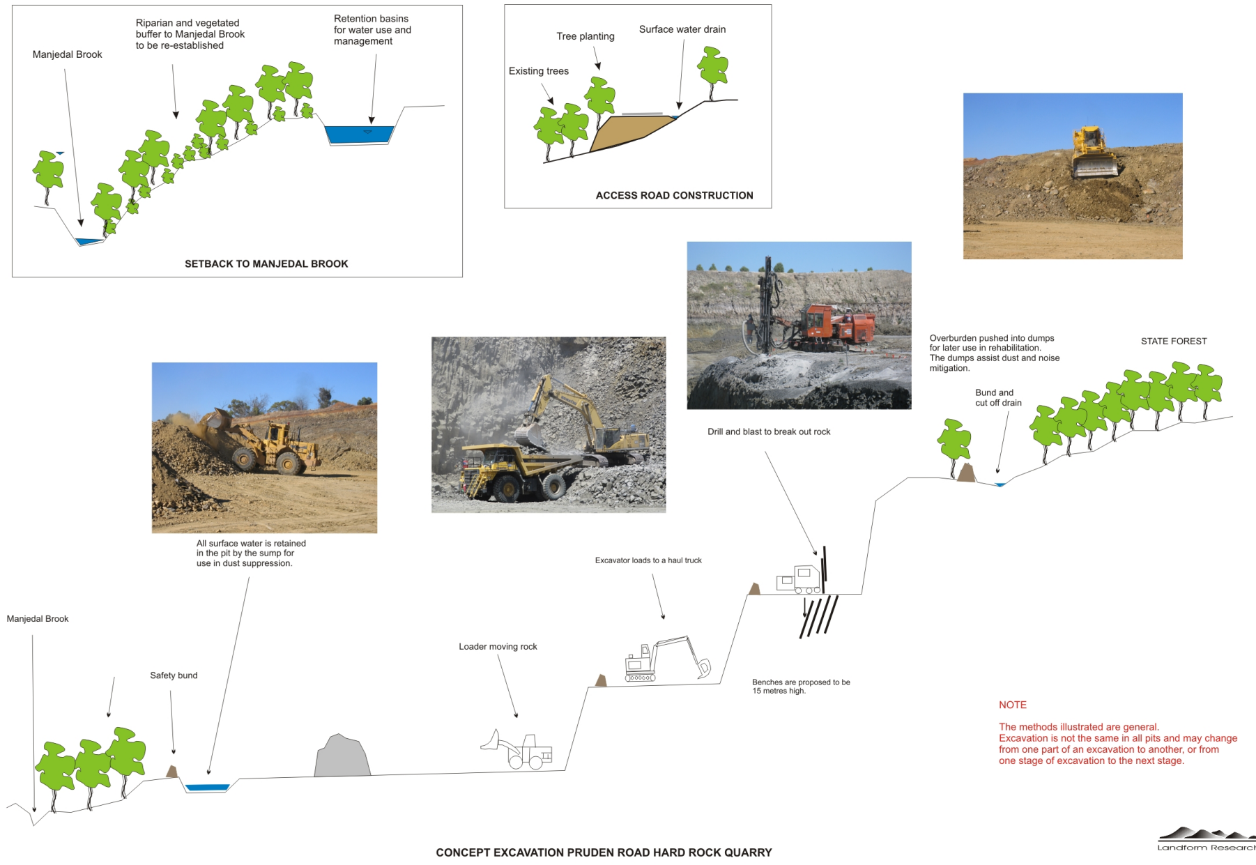
Figure 1 – 8 Concept and sketch section of pit operations
