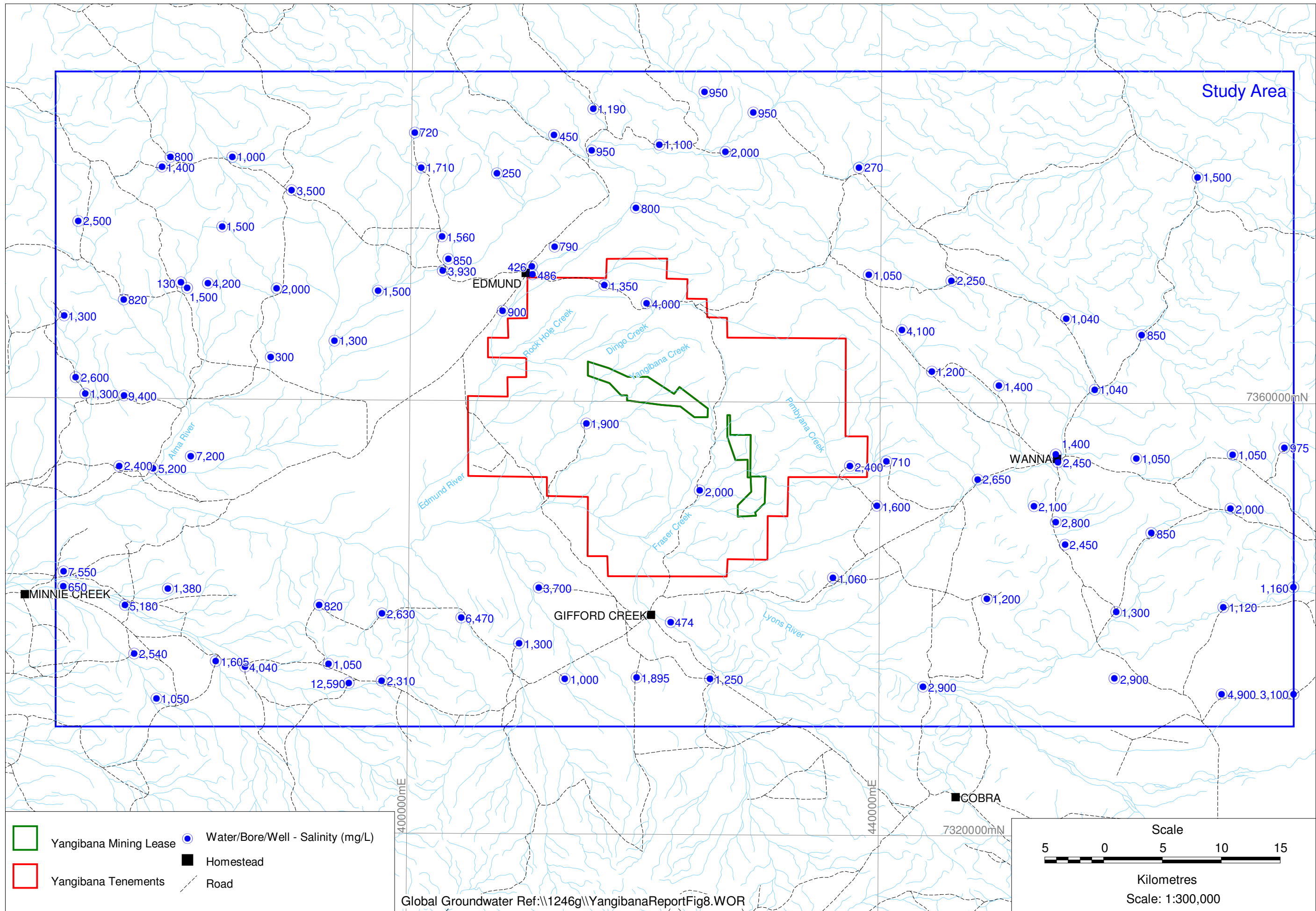
Figure 8. Groundwater Salinity
