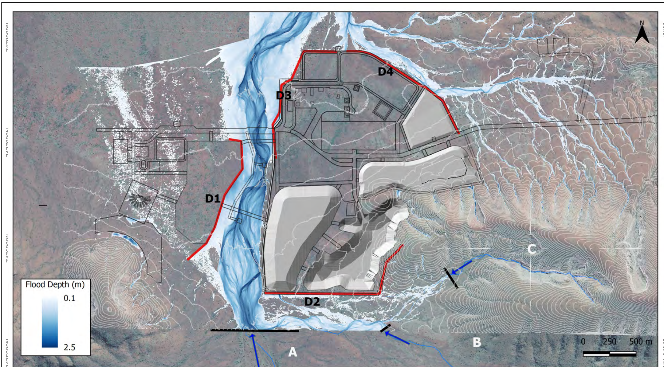
AQ2 Figure 4.3: Mine Creek Post-development 1% AEP Flood Map Revised Infrastructure
