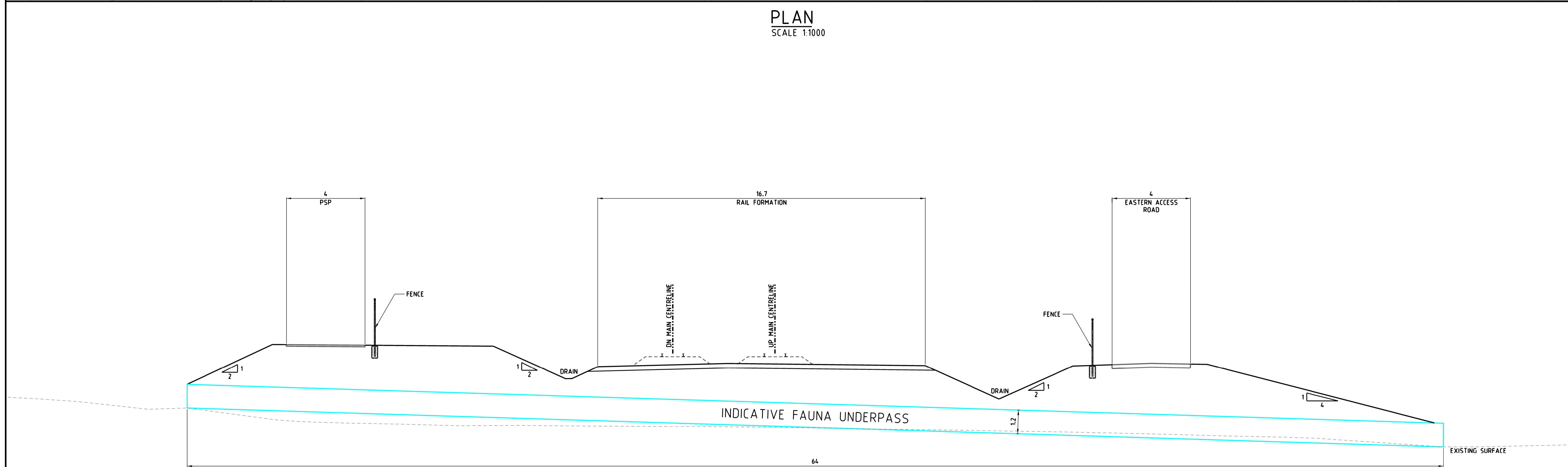
SECTION SCALE 1:100
