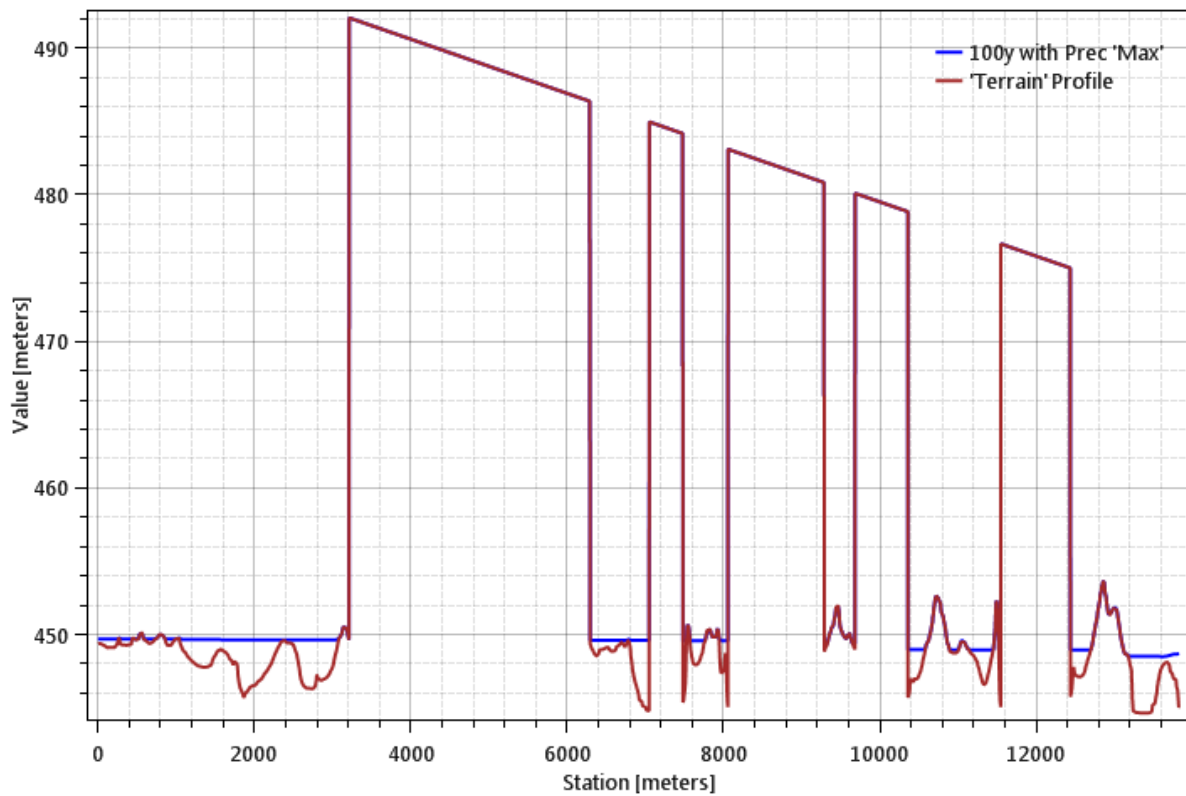
Water Surface Profiles Along E3: 0.01 AEP Flood
