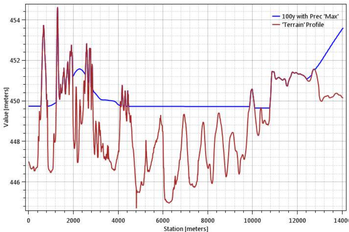
Water Surface Profiles Along E1: 0.01 AEP Flood
