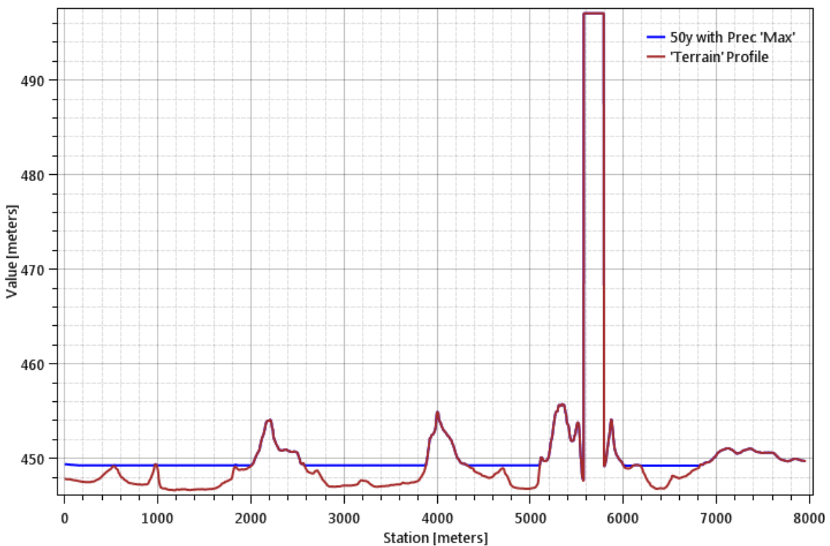
Water Surface Profiles Along N1: 0.02 AEP Flood
