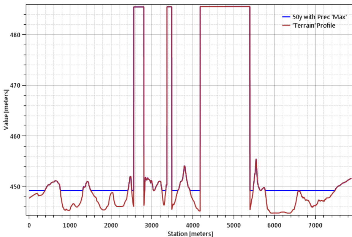
Water Surface Profiles Along N2: 0.02 AEP Flood
