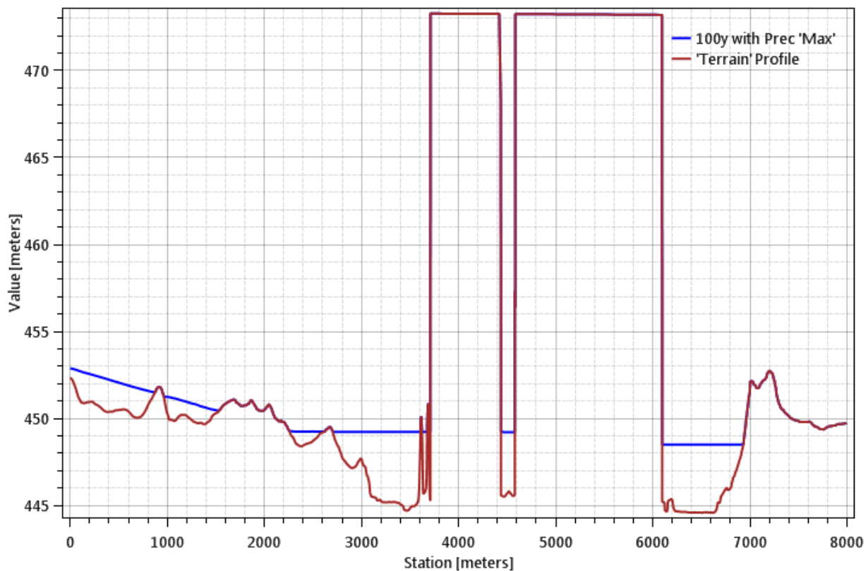
Water Surface Profiles Along N3: 0.01 AEP Flood
