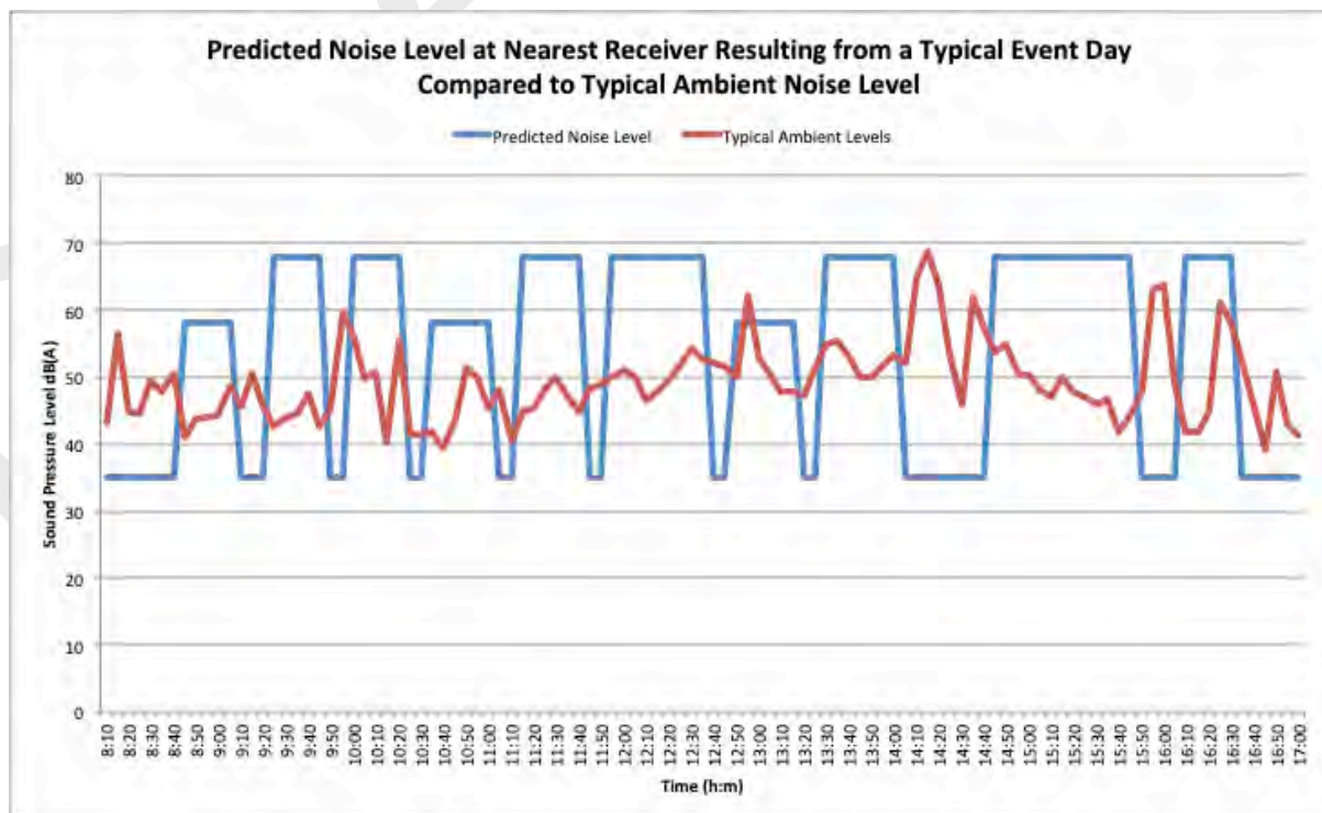
Figure 6-1 Noise Predictions from Typical Major Event Compared to Ambient Noise Levels
