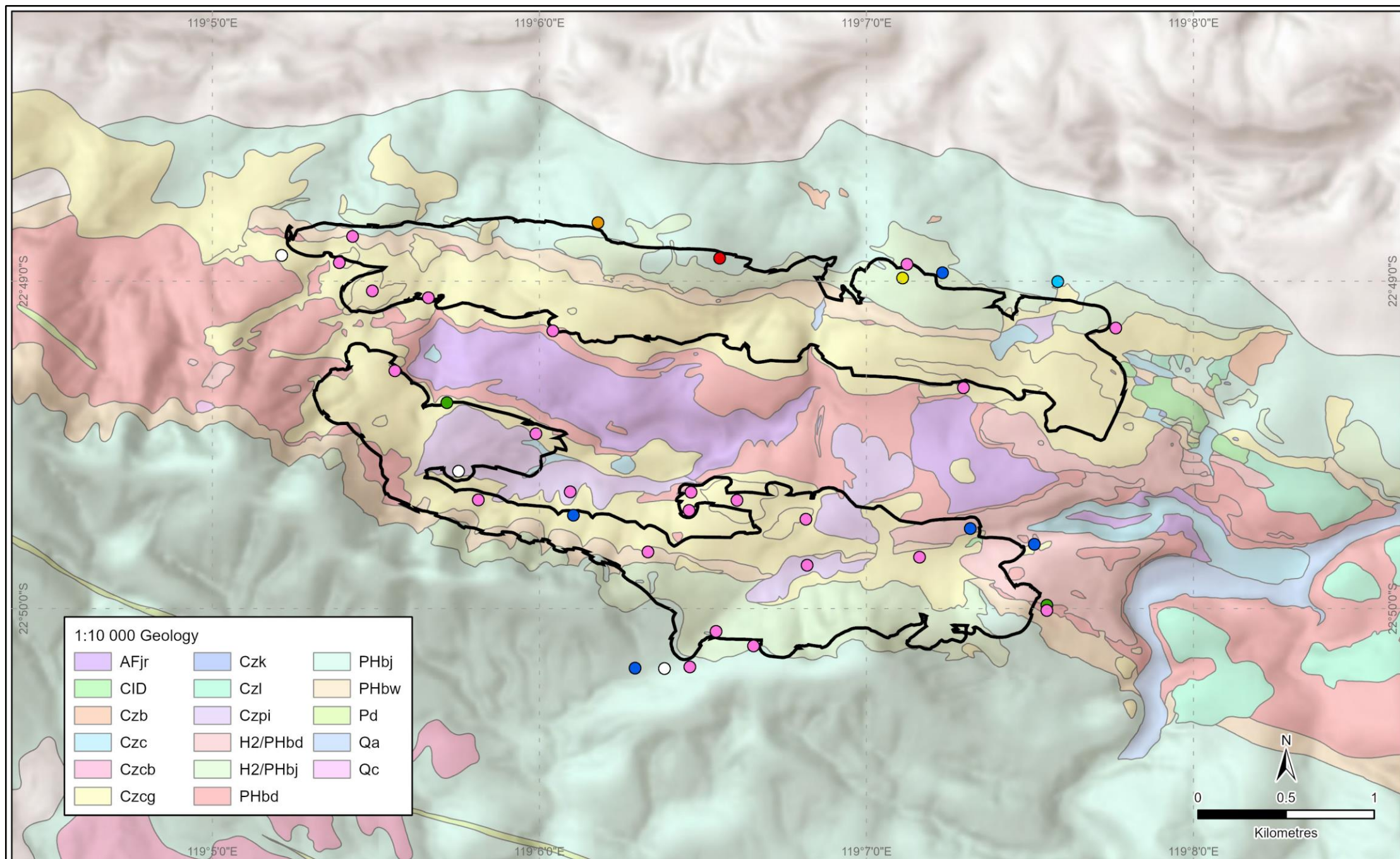
Figure 11. Distribution of Opiliones, Palpigradi and Pseudoscorpiones recorded around the Ministers North pits
