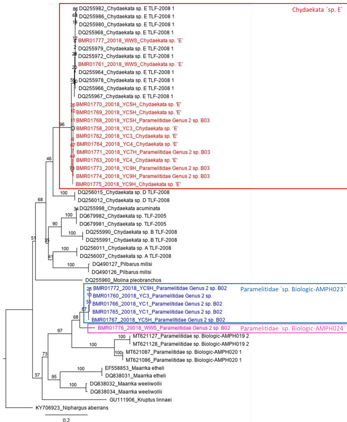
Figure 3.1.1: Maximum Likelihood phylogeny, with bootstrap values.
