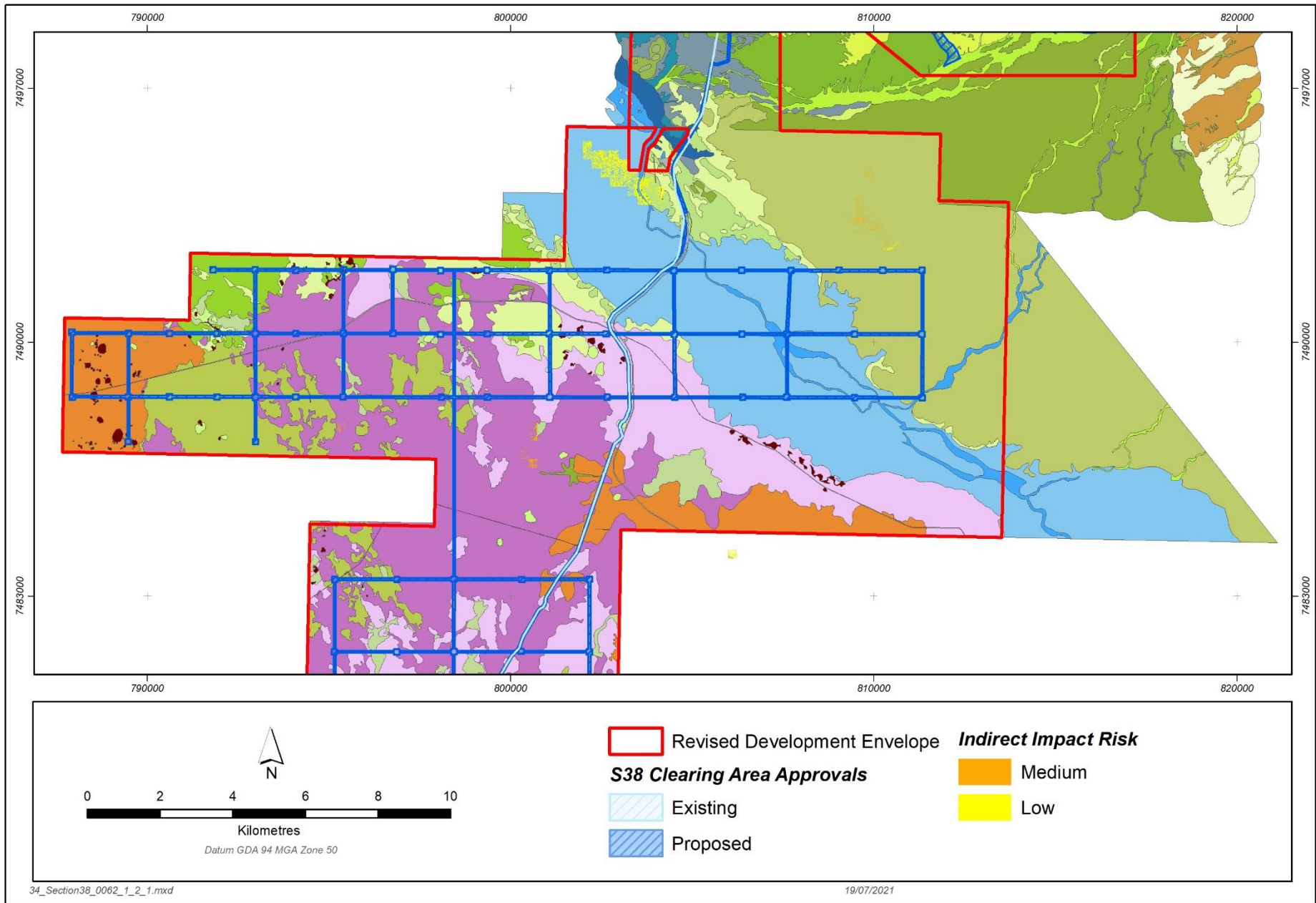
Figure 4-13: Vegetation Units across the Revised Development Envelope Remote MAR Area
