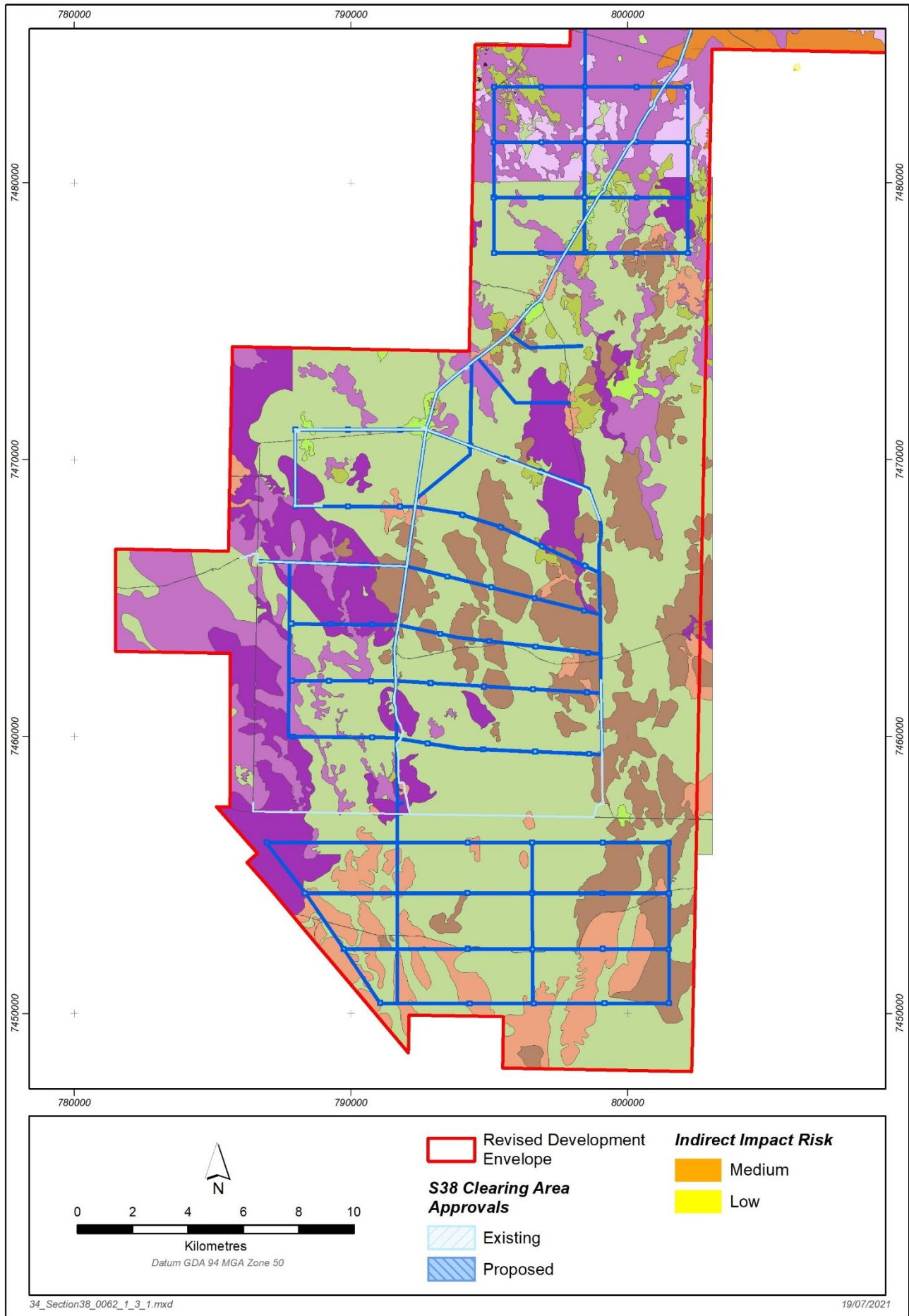
Figure 4-14: Vegetation Units across the Revised Development Envelope Southern Borefield Area
