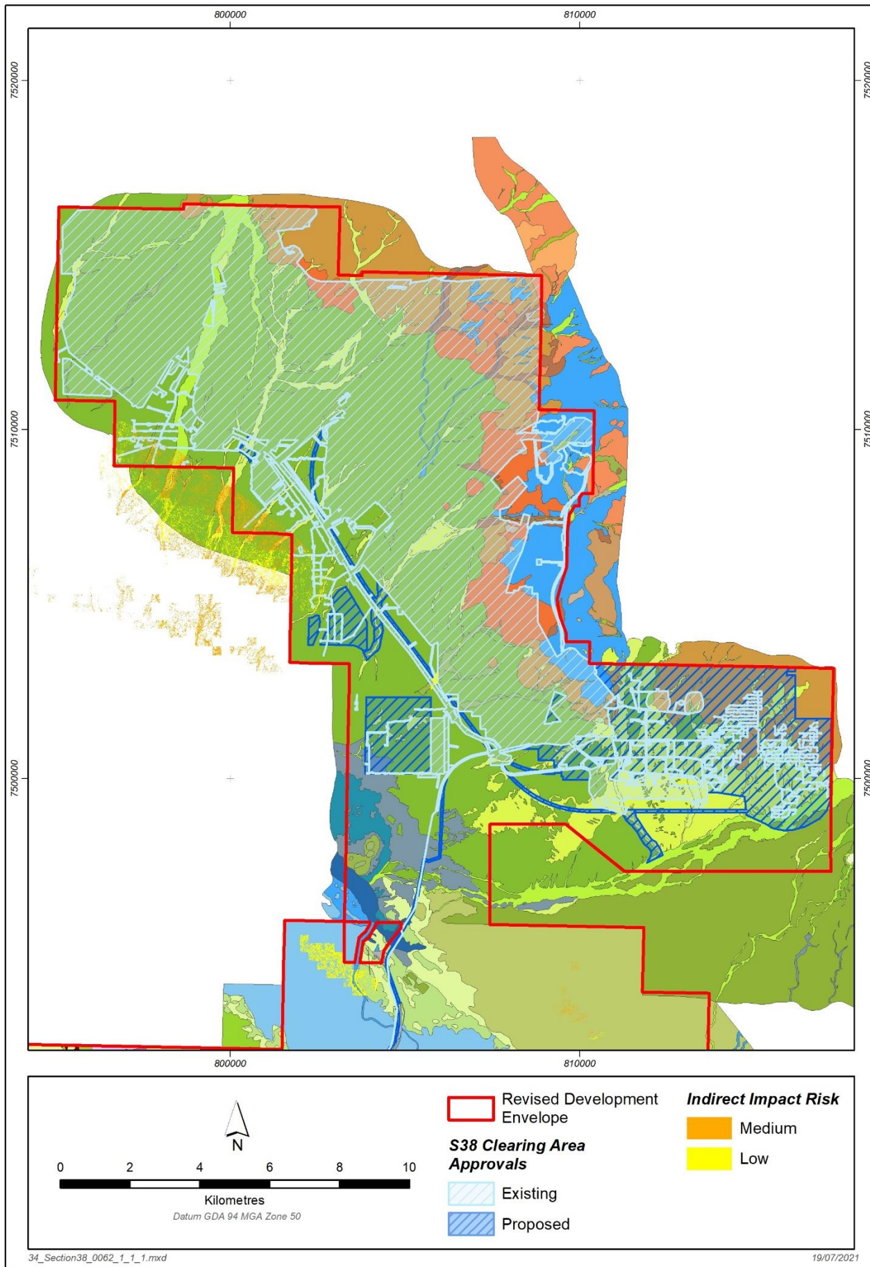
Figure 4-12: Vegetation Units across the Revised Development Envelope Mine Area
