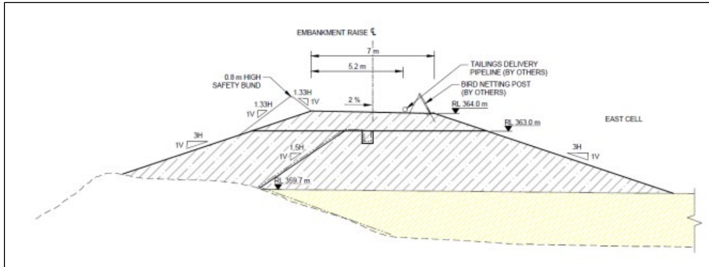
Figure 5-86: Gidji II typical cross section of 4m high upstream wall raise on Gidji II TSF (with liner detail;2022)
