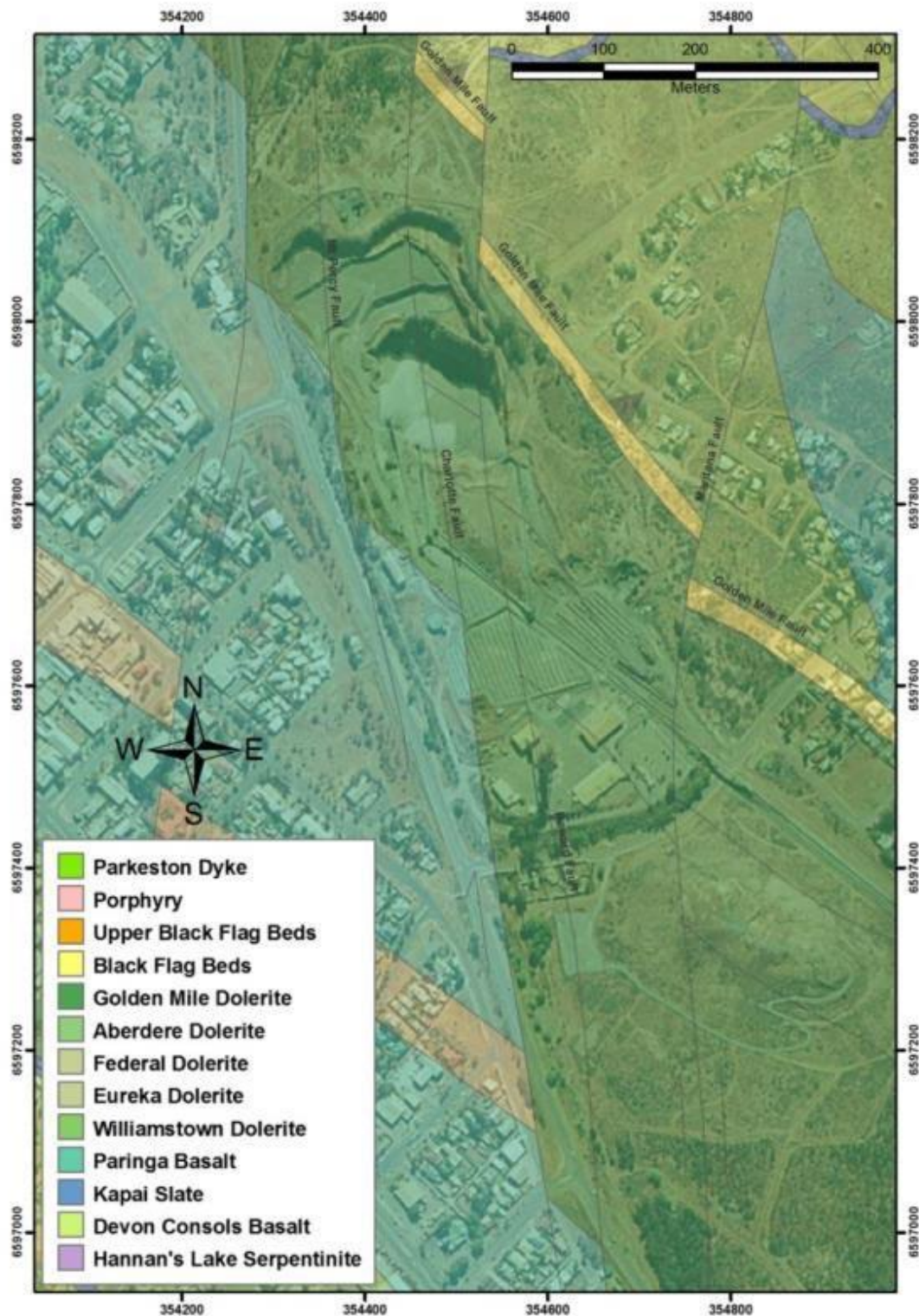
Figure 5-6: Mt Charlotte Lithology
