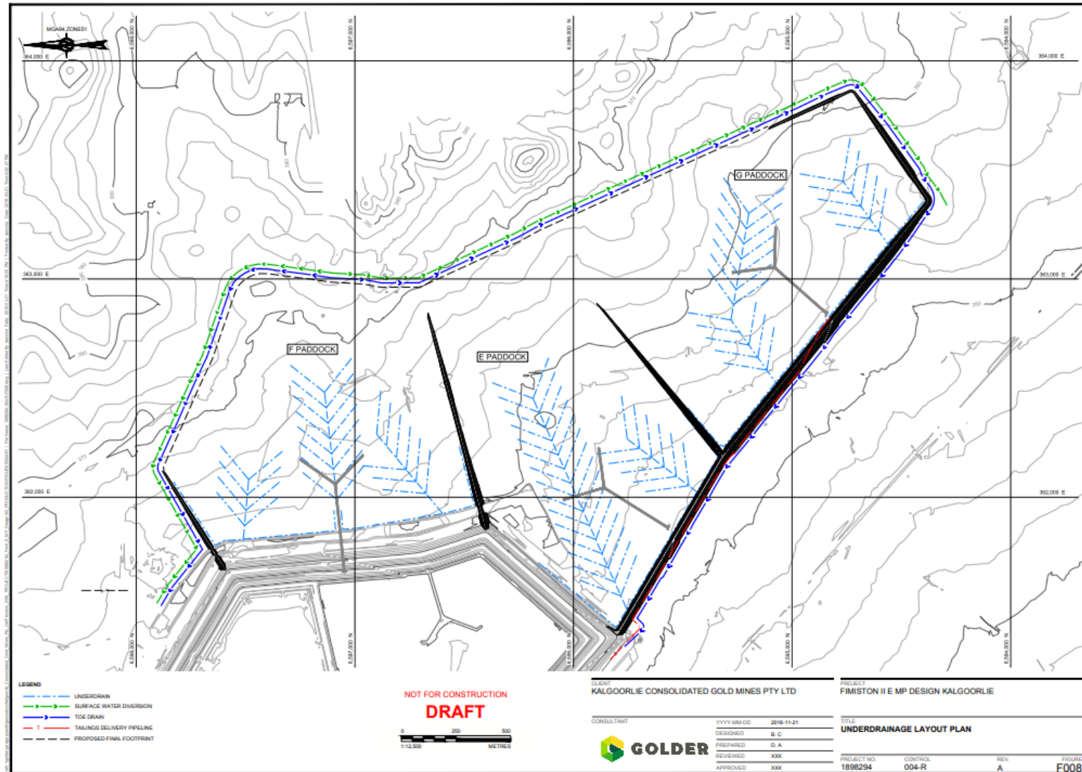
Figure 5-73: Plan view of Fim IIE TSF showing underdrainage system
