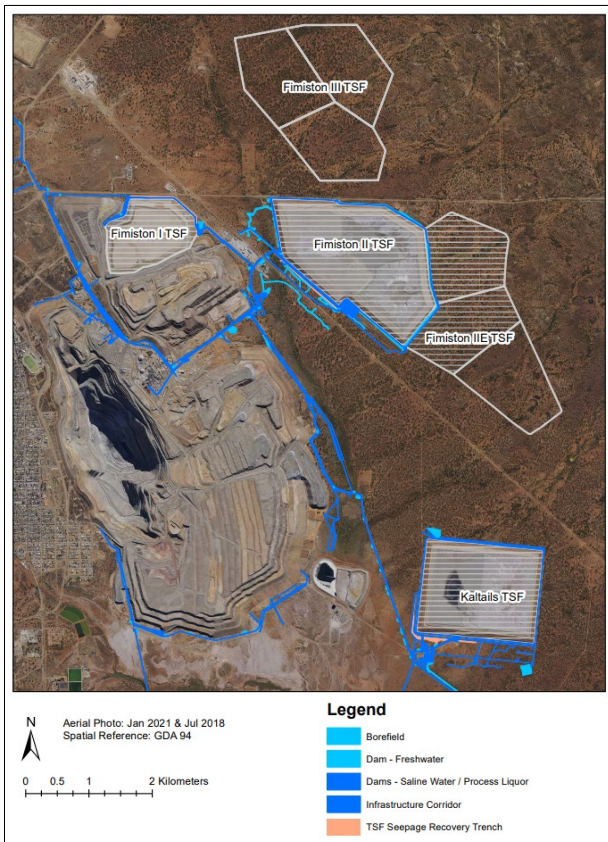
Figure 5-79: Water Containment Facilities Domain and Site Dams Feature
