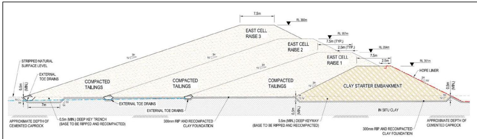
Figure 5-85: Gidji II typical cross section of outer embankment walls (downstream construction)
