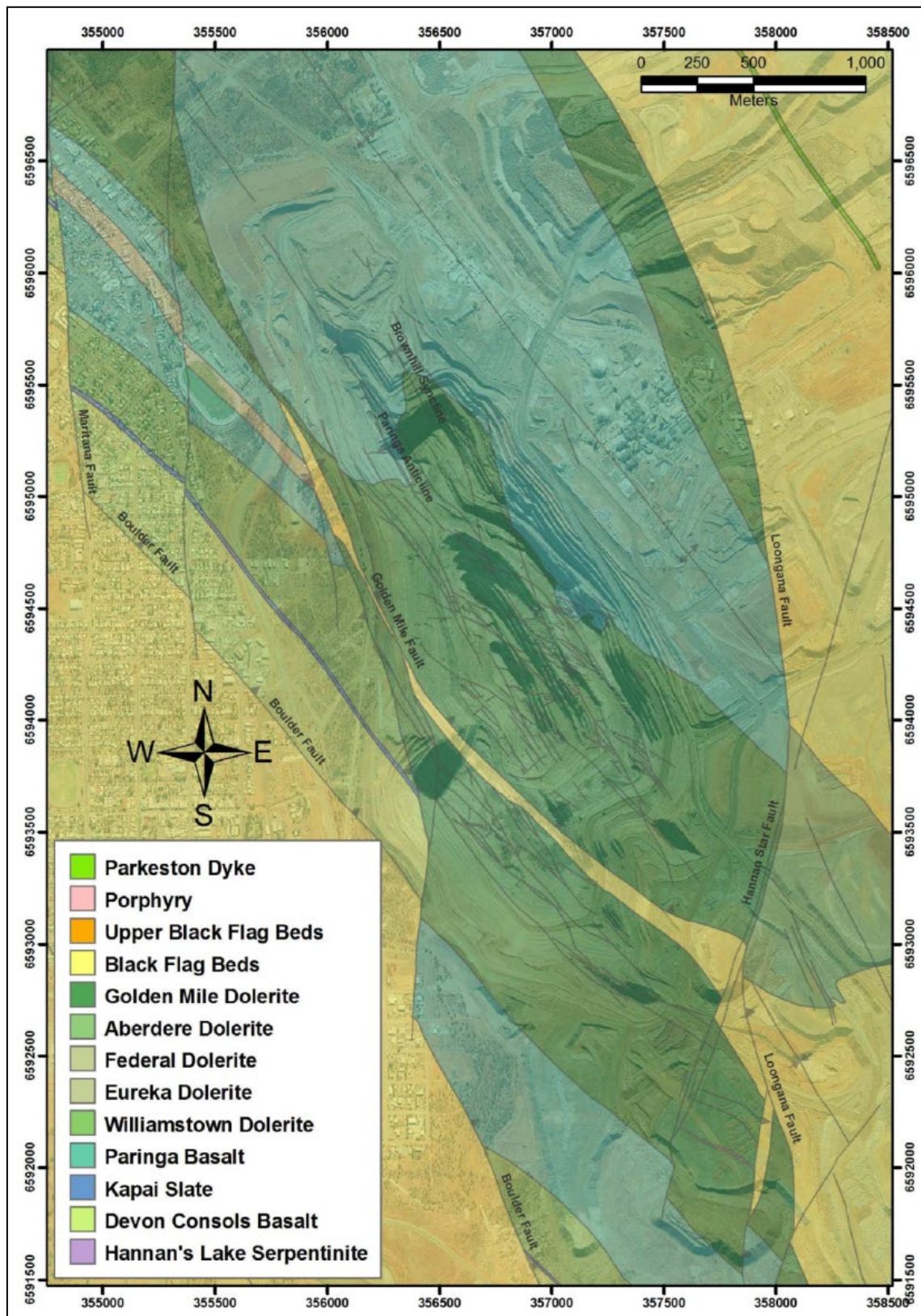
Figure 5-4: Fimiston Lithology
