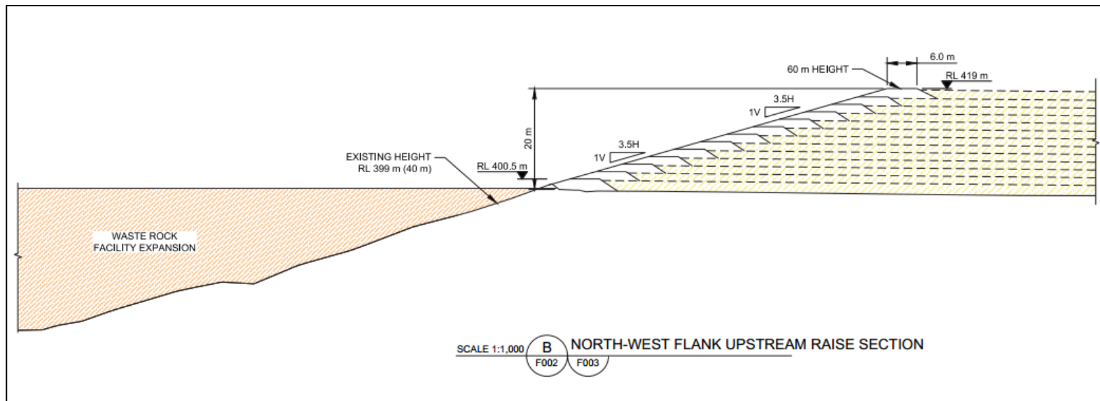
Figure 5-62: Fimiston I TSF Cross-sectional View
