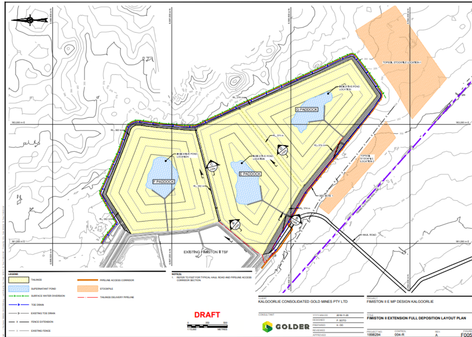
Figure 5-72: Plan view of Fim IIE TSF
