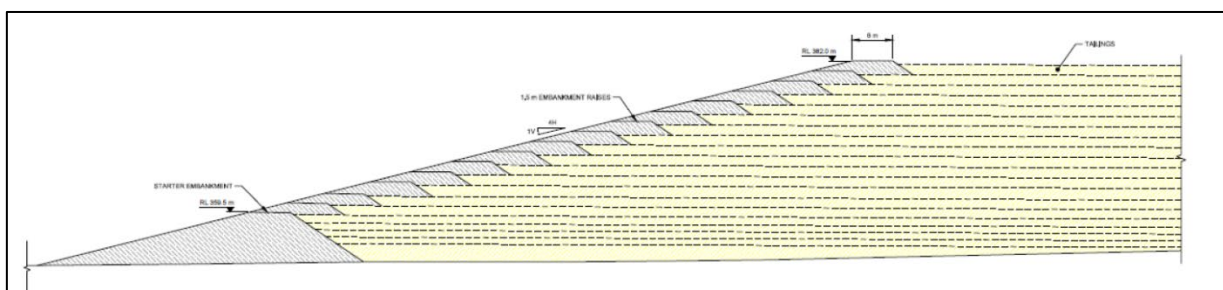
Figure 5-71: Typical cross section for Fim IIE TSF
