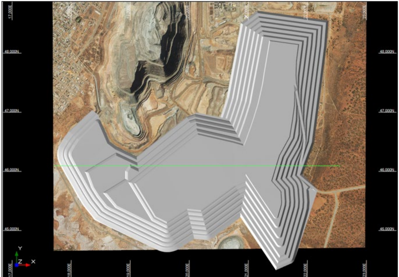
Figure 5-25: Proposed Southern WRD Design (mine site grid)
