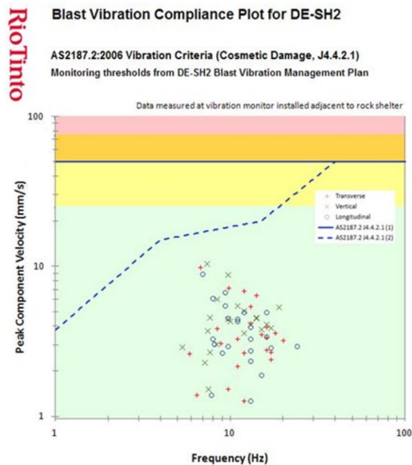
Figure 2. Example of Blast vibration data from West Angelas Deposit E rock shelter
