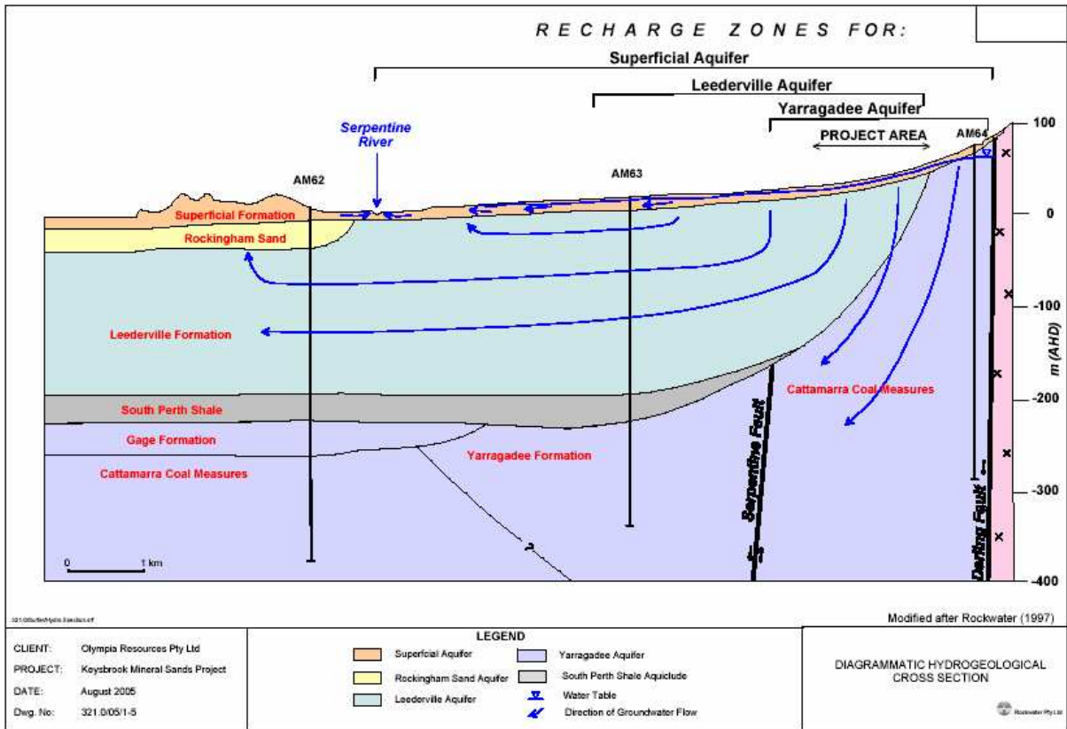
Figure 6: Diagrammatic Hydrogeological Cross-Section of the Swan Coastal Plain
