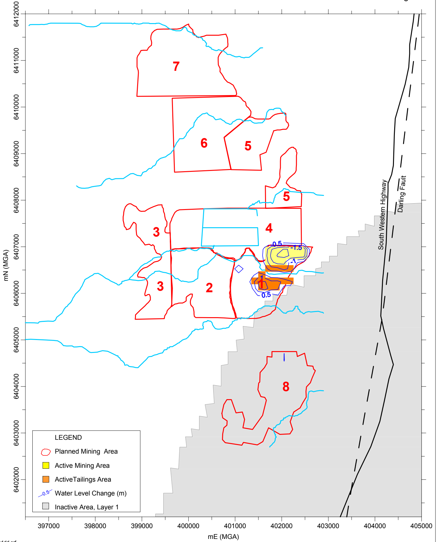
Figure 20 - Dewatering Drawdown
