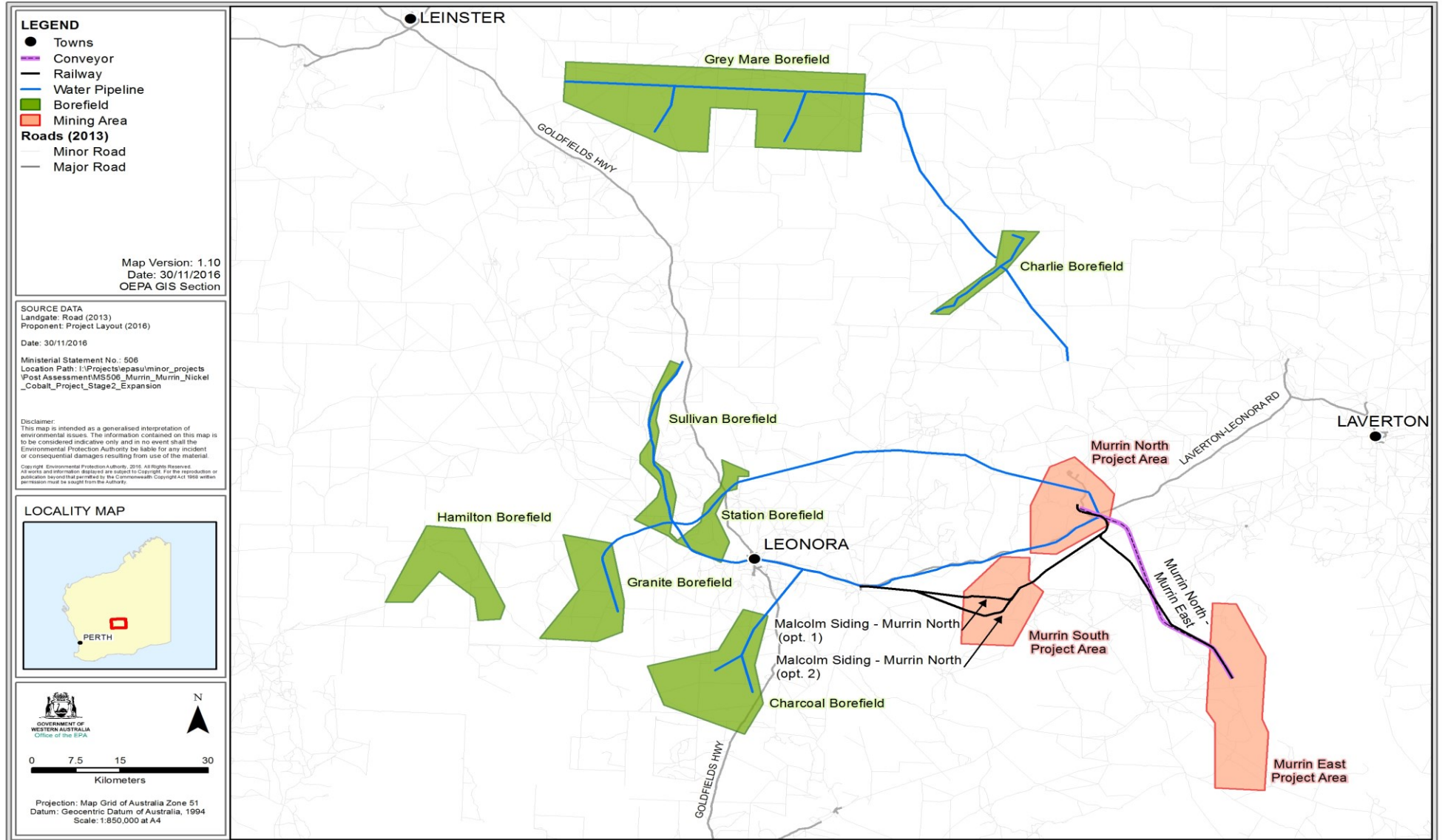
Figure 2 Murrin Murrin Project Layout
