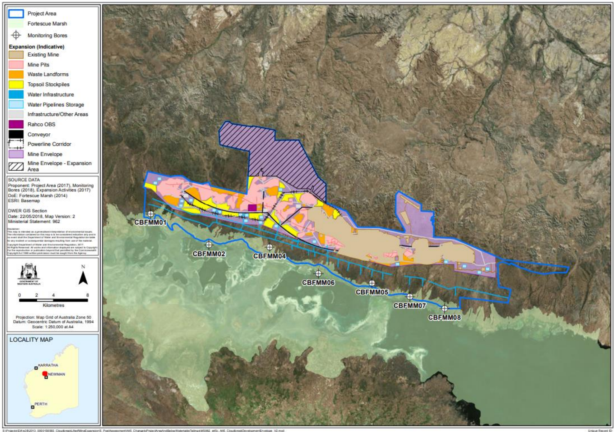
Figure 2: Proposal's Mine Envelope (including Northern Tenements Expansion area) and location of monitoring bores
