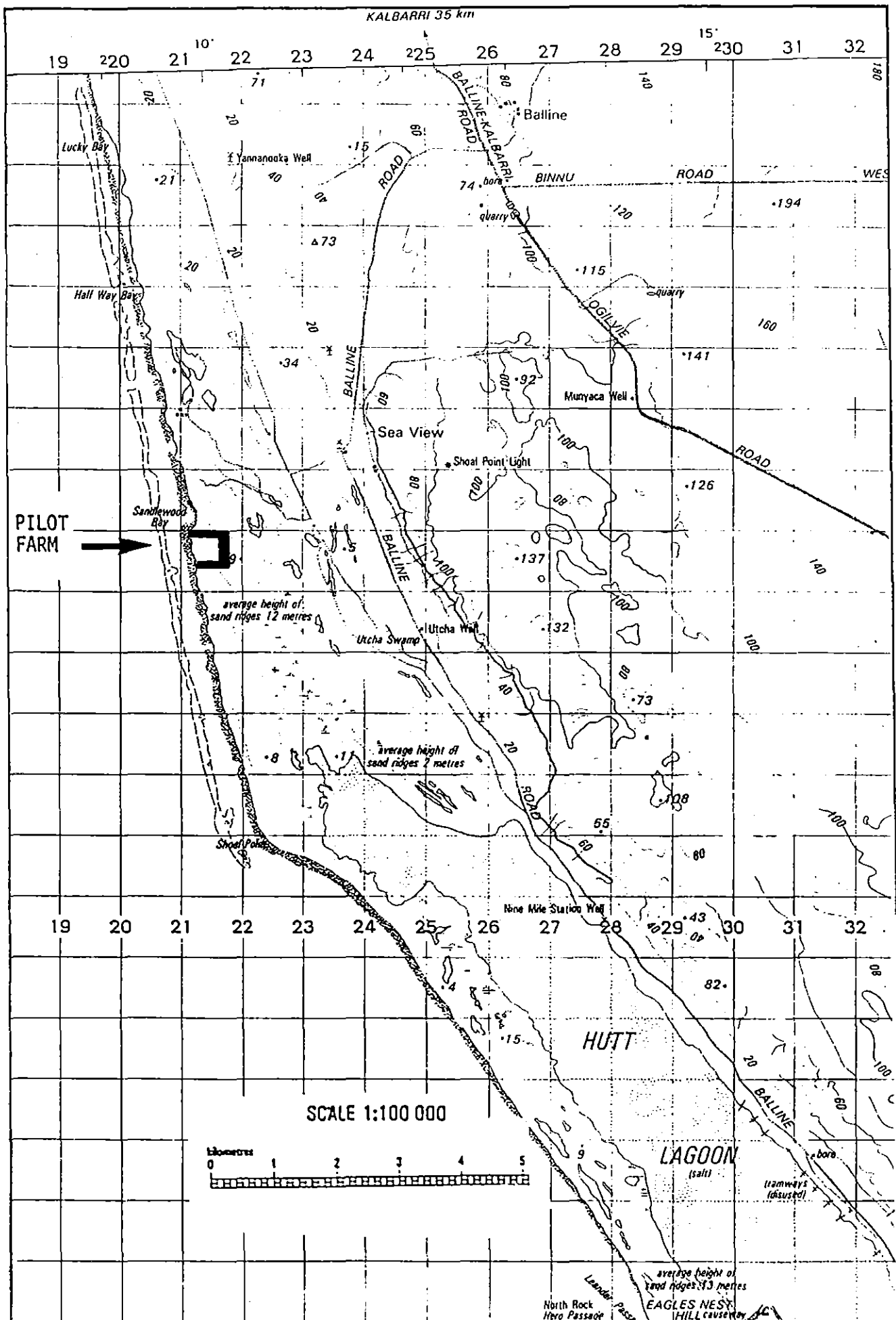
Figure 1. Location of Proposed Pilot Plant
