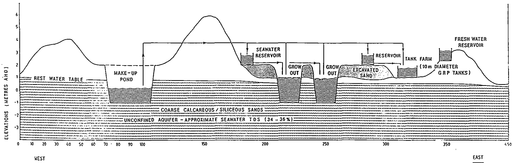
Figure 2. Cross Section of Proposed Pilot Plant (from Southern Seas Farms Ltd)
