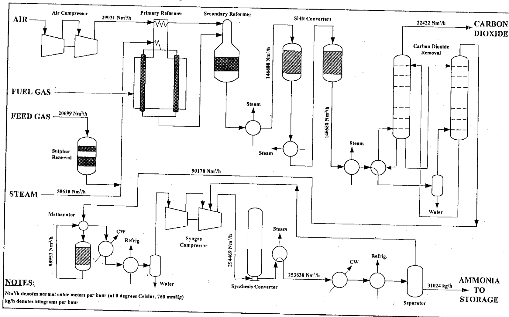
PROCESS FLOW CHART Figure 5
