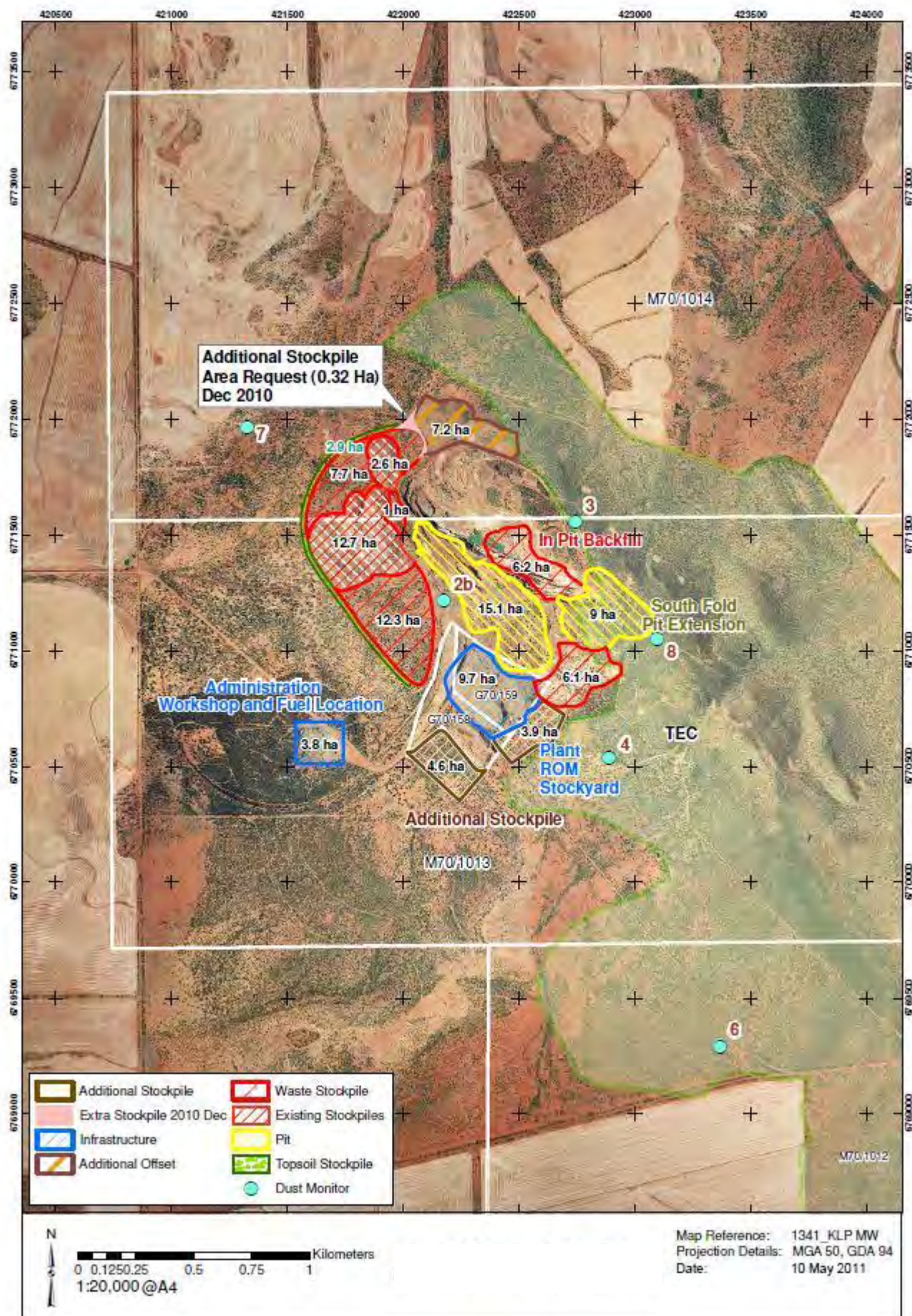
Figure 1 - Koolanooka Site Plan
