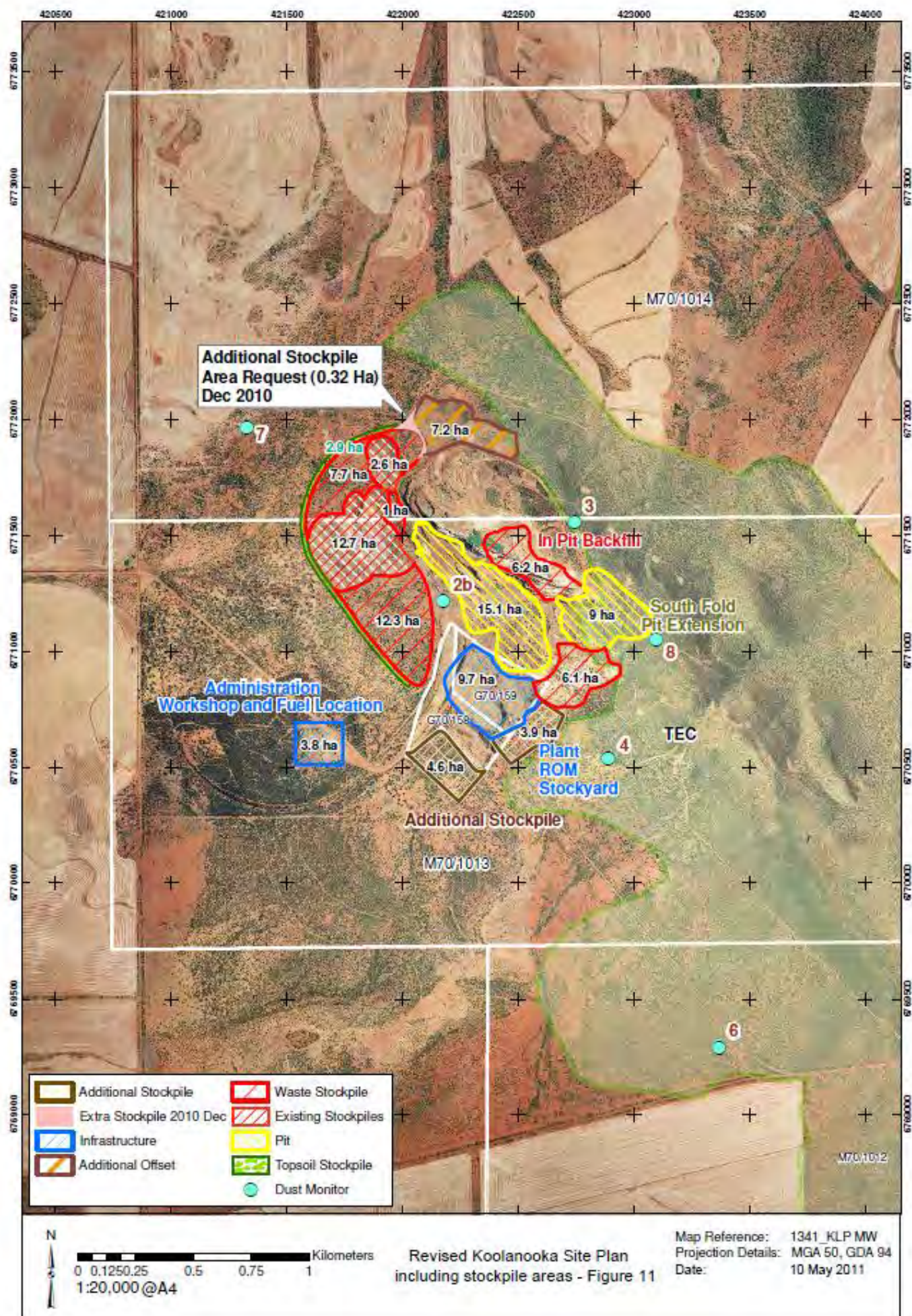
Figure 11 Revised Koolanooka Site Plan including additional stockpile areas
