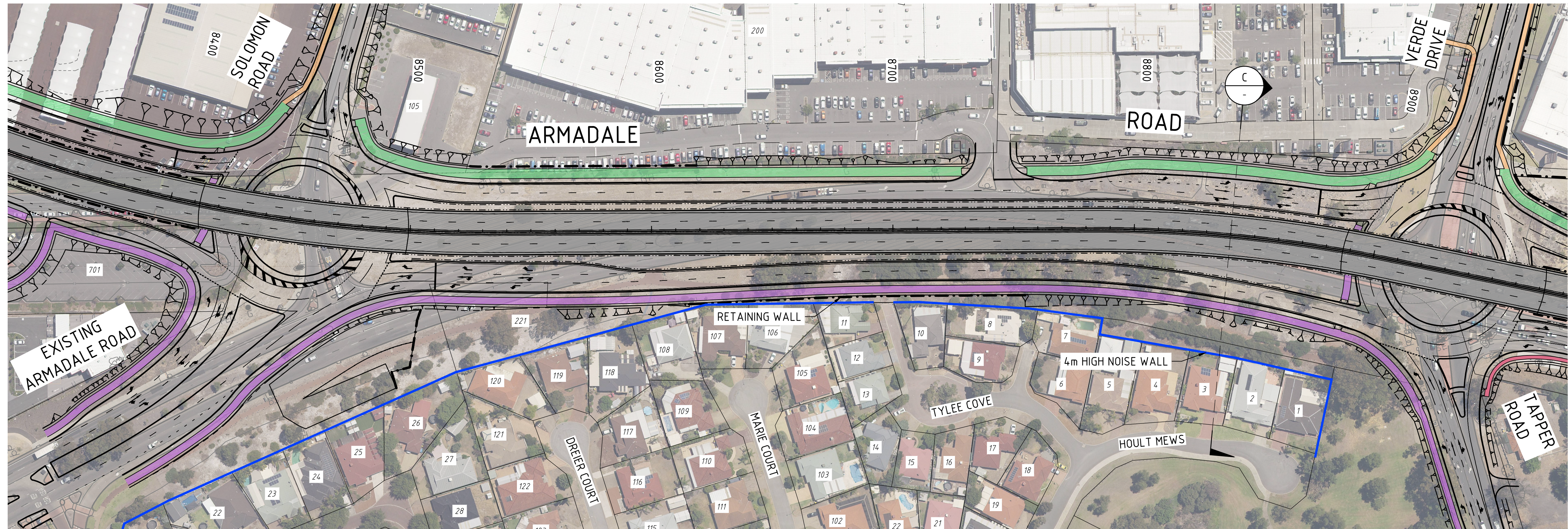
PLAN SCALE 1:1000
