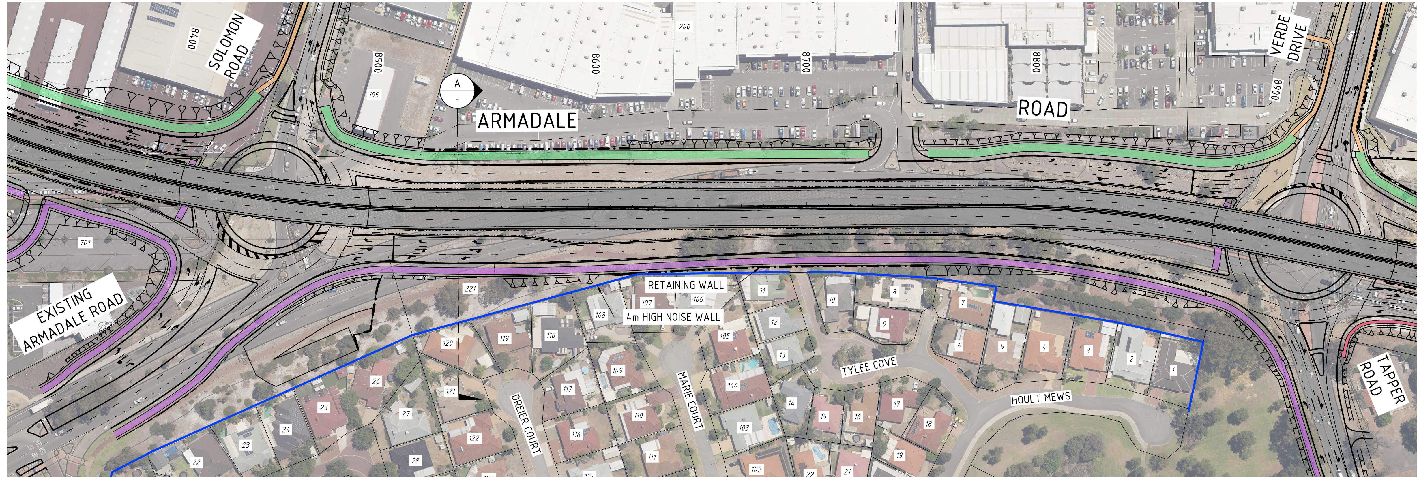
PLAN SCALE 1:1000
