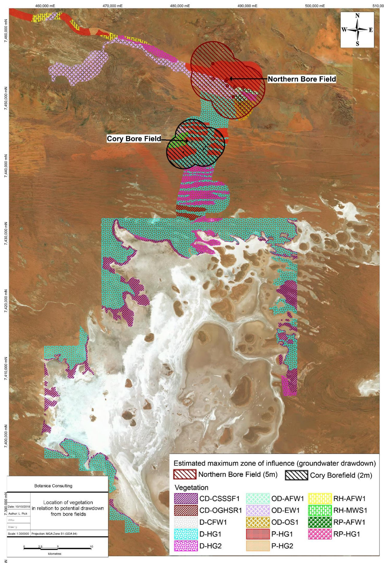
Figure 6-5: Vegetation in relation to Bore Fields potential zone of influence (groundwater drawdown)
