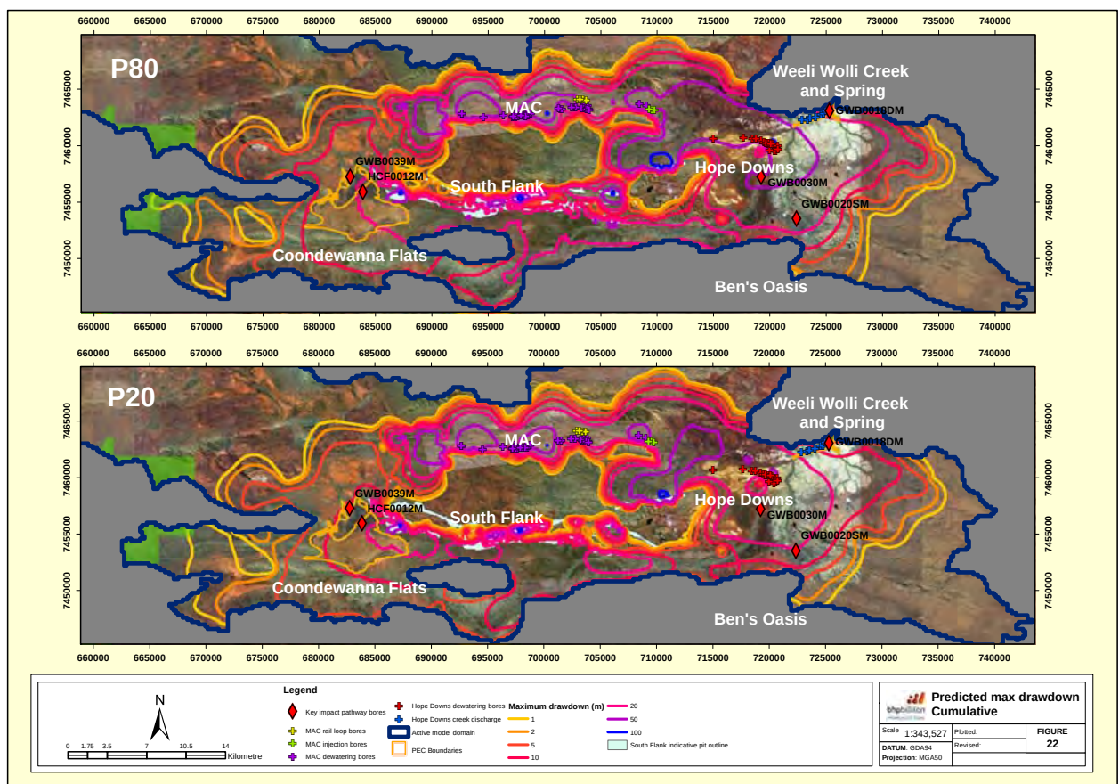
Figure 9: Cumulative P80 and P20 drawdown scenarios
