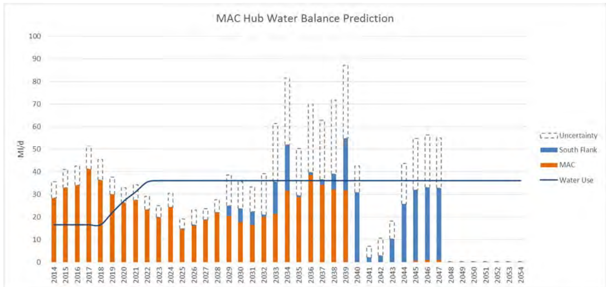
Figure 5: Combined Mining Area C water balance showing annual dewatering estimates compared with water demand
