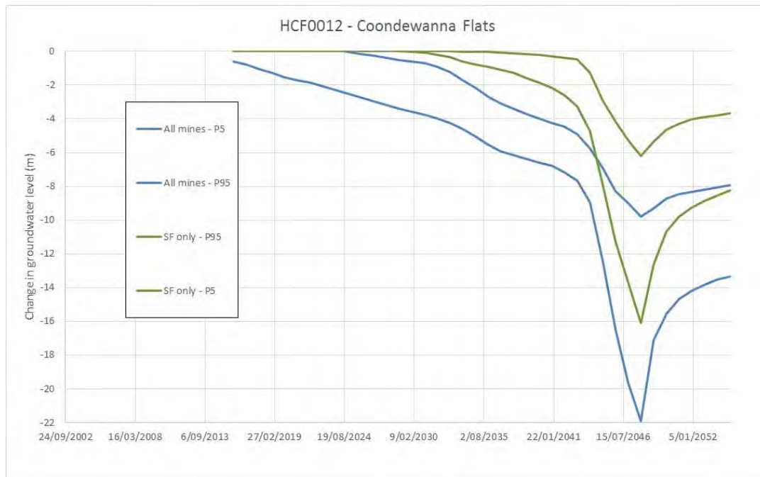
Figure 10: Predicted drawdown and recovery at HCF0012.
