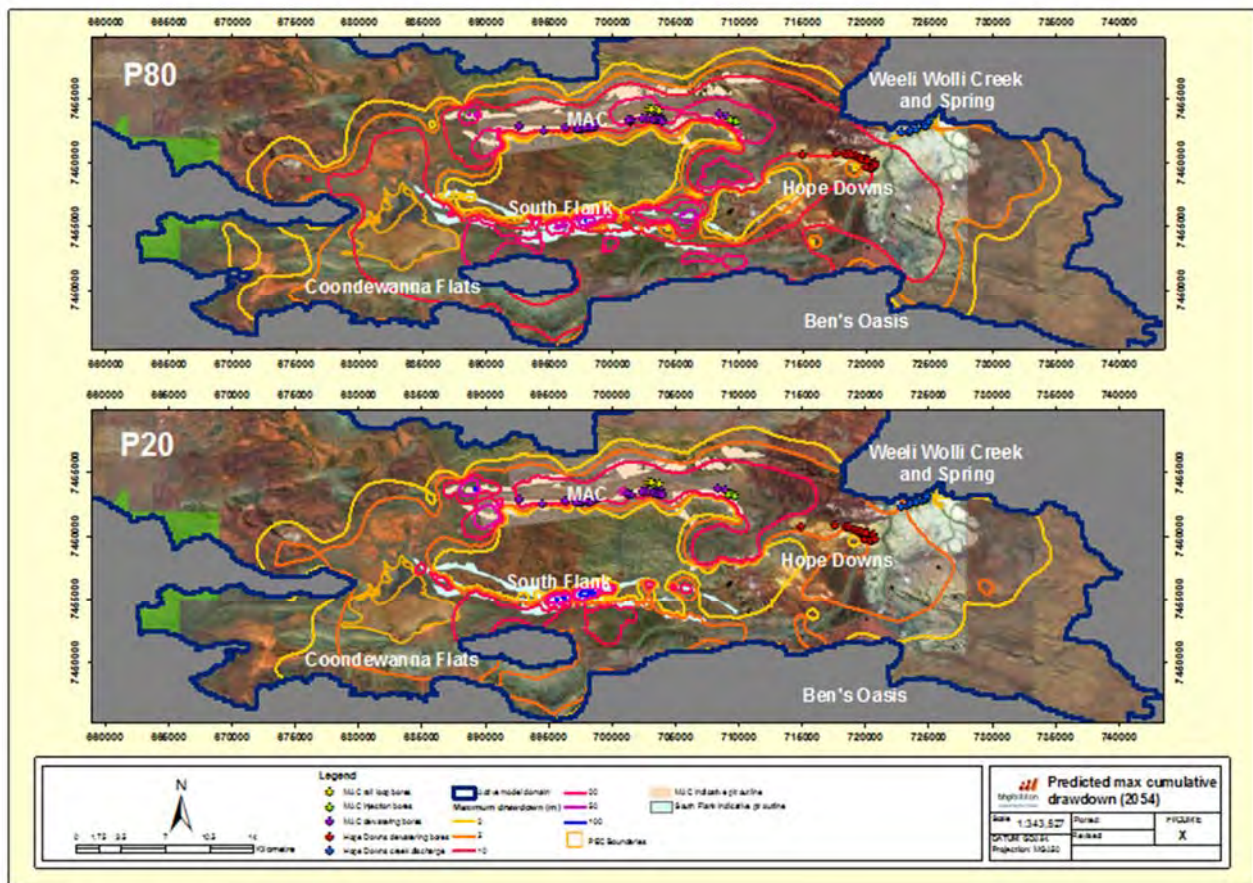
Figure 7: Cumulative Drawdown in 2054
