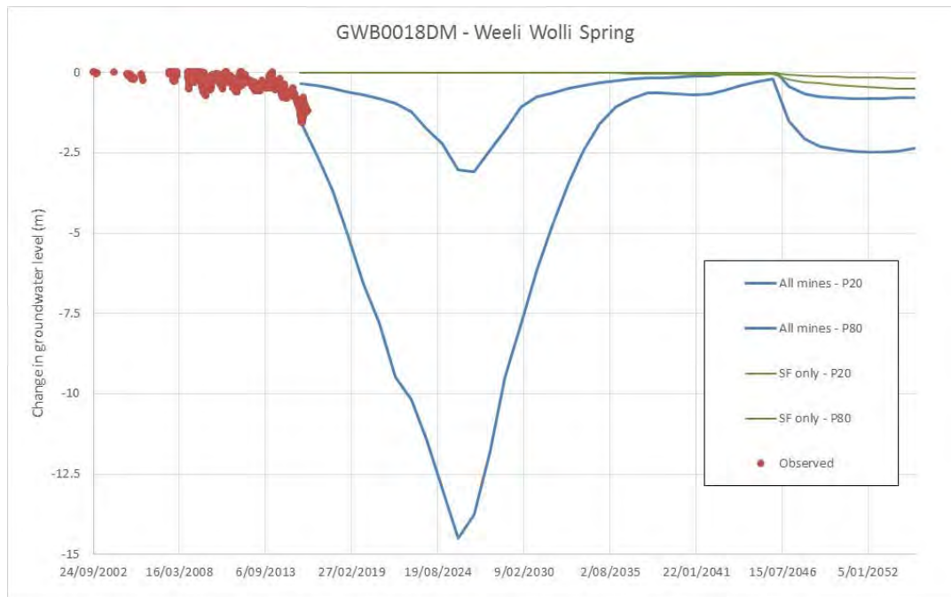
Figure 11: Predicted drawdown and recovery at GWB0018
