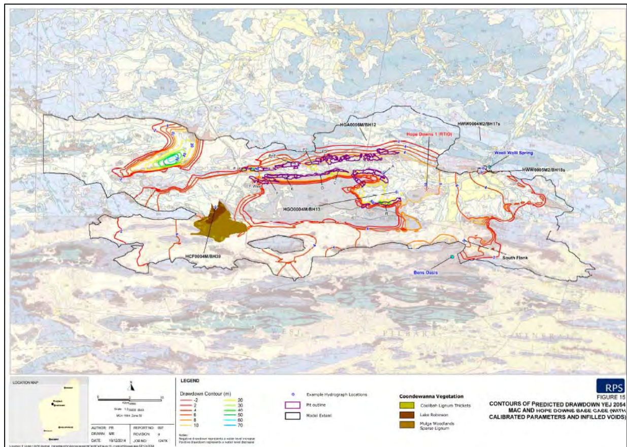
Figure 6: 2054 Drawdown Footprint from EMP Rev 6 Proposal
