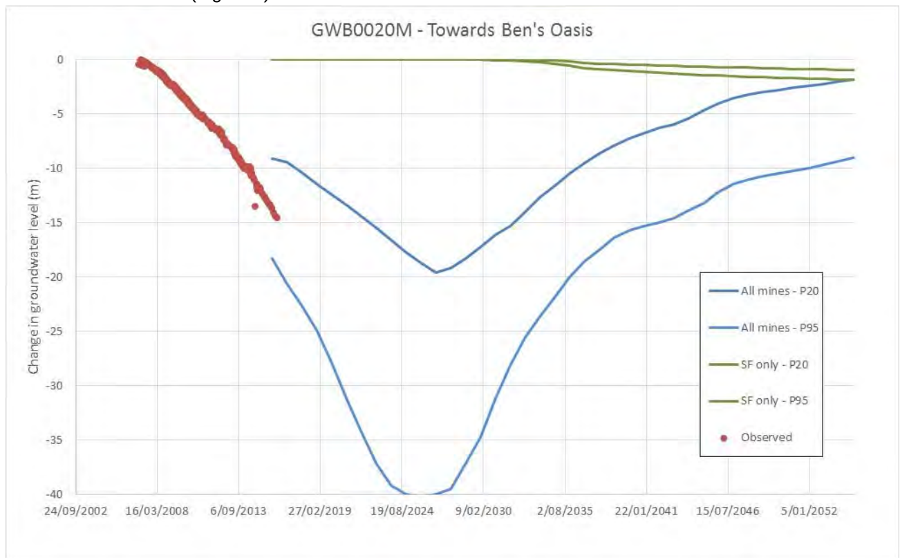
Figure 12: Modelled drawdown and recovery at GWB0020
