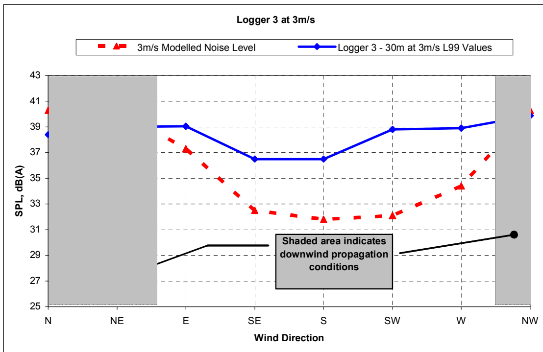
Figure 3: Southern Monitor (Logger 3 Boundary Rd) Measured v Predicted SPL's
