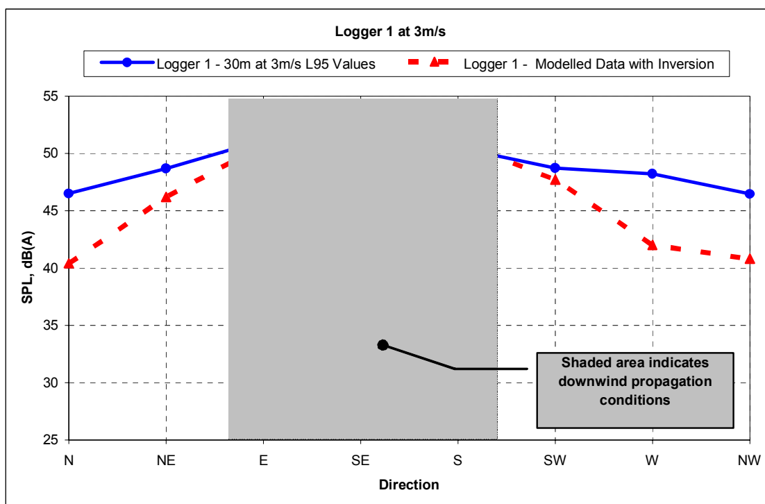
Figure 1: Northern Monitor (Logger 1 Access Rd) Measured v Predicted SPL's
