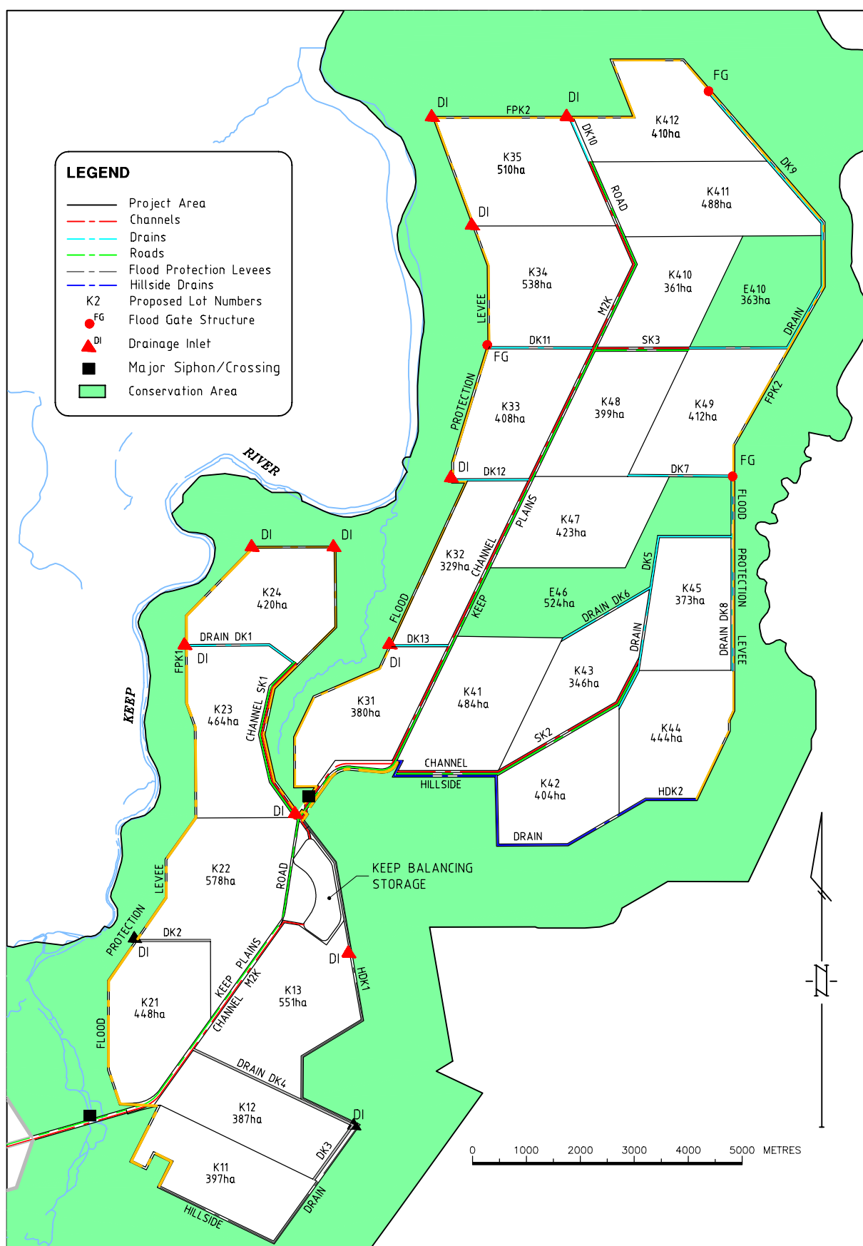
Figure 3.5 Infrastructure - Keep River Plain
