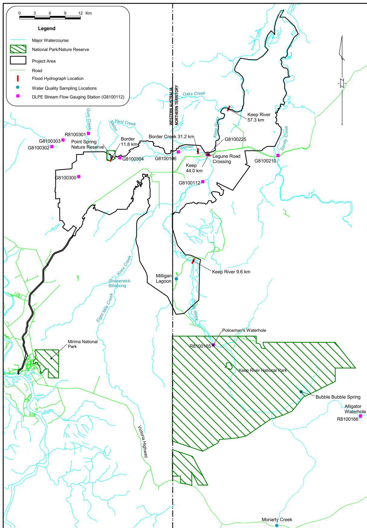
Figure 5.1 Regional Hydrology
