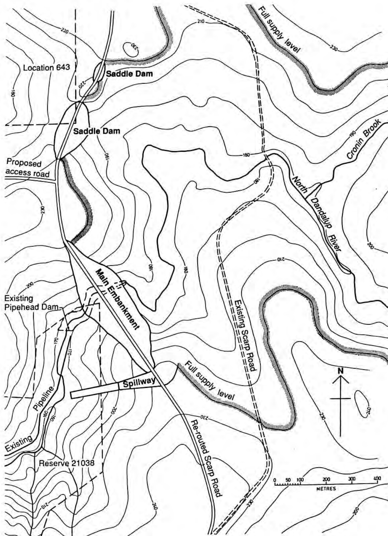
Figure 8: North Dandalup Dam; Plan of Works
