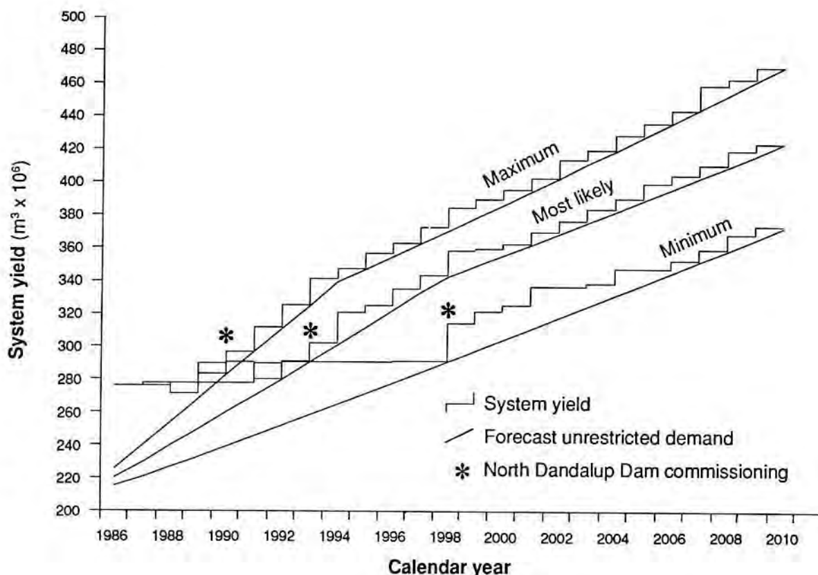
Figure 2: Source Development Timetables (for 'maximum', 'most likely' and 'minimum' demand estimates)
