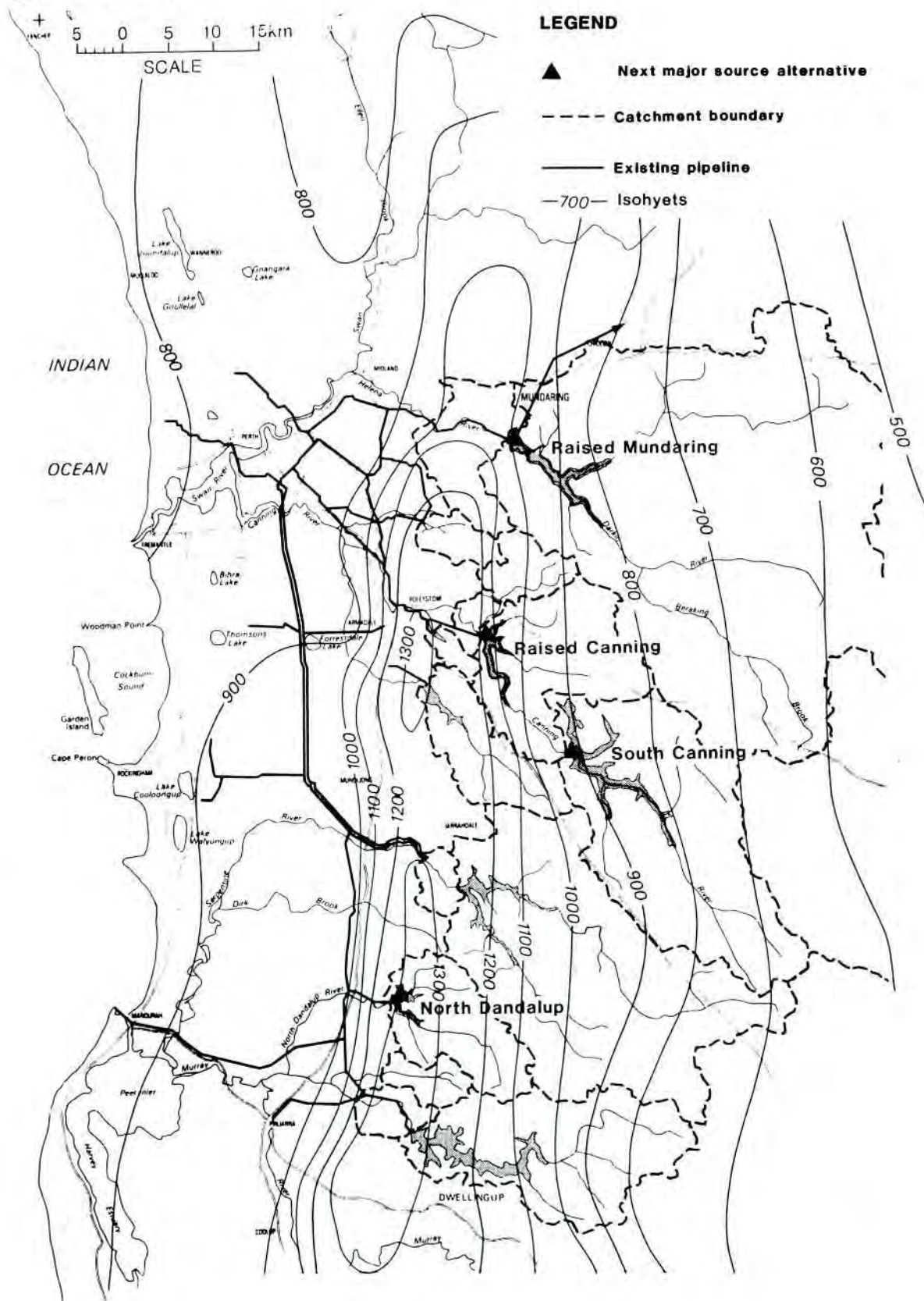
Figure 3: Alternatives for the Next Major Water Supply Source for Perth
