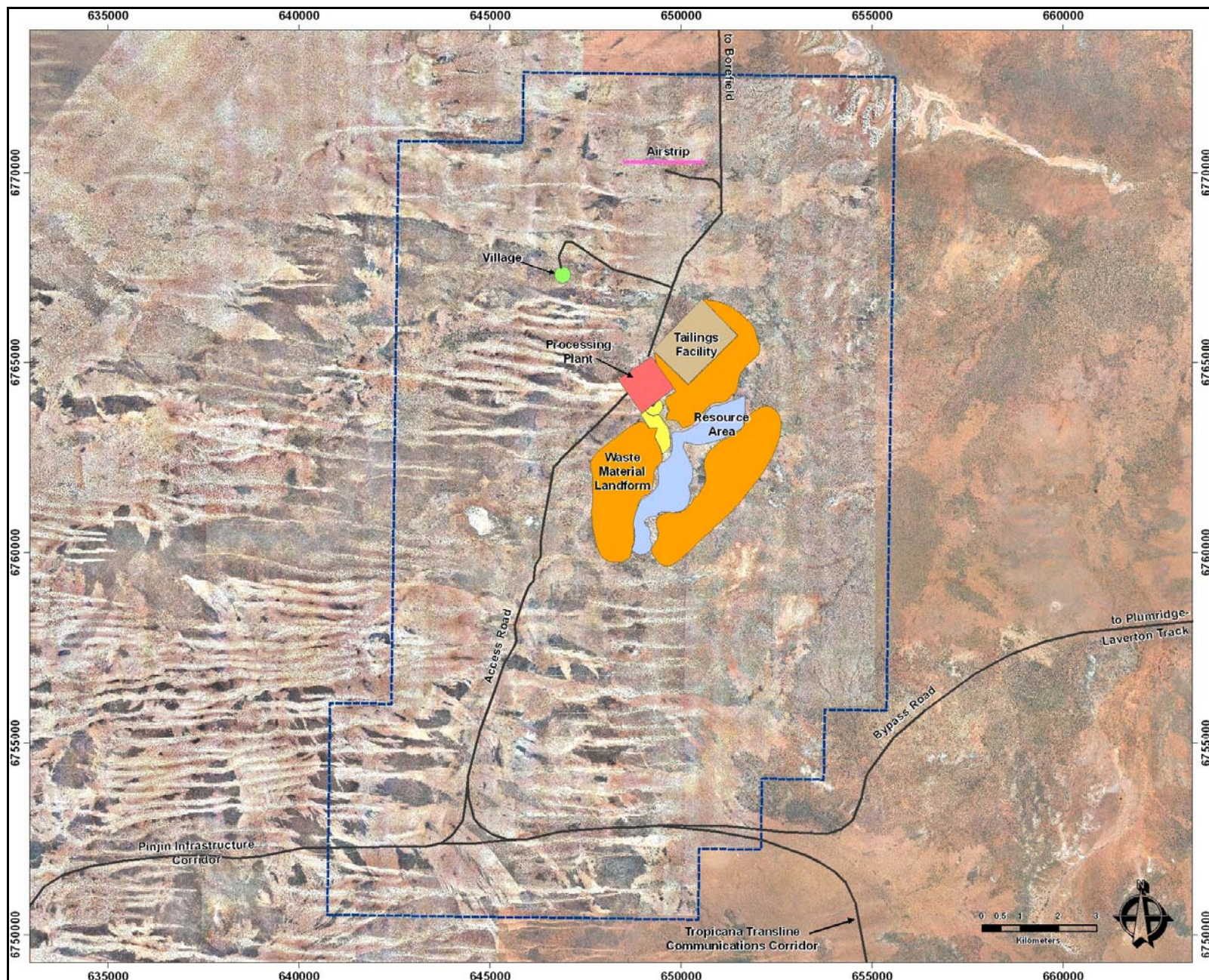
Figure 2: Project footprint and layout of key components
